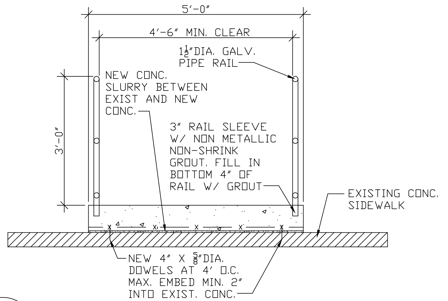
2 NEW RAMP TRANSVERSE SECTION A4 3/4" = 1'-0"
