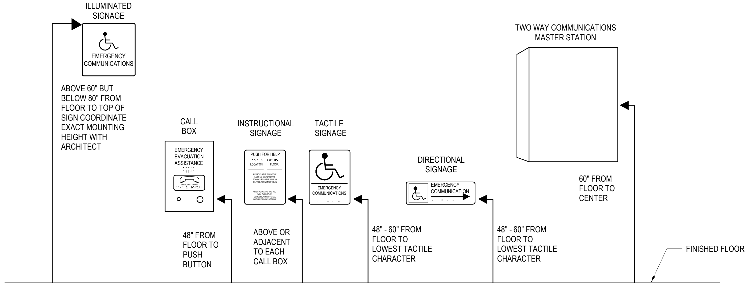
C3 TWO WAY COMMUNICATIONS MOUNTING HEIGHT DETAIL NTS
