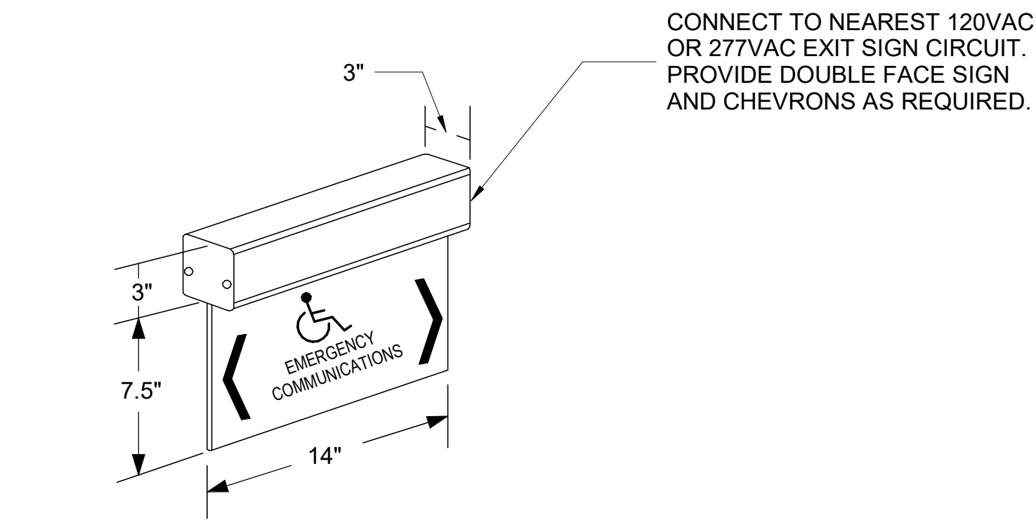
C1 TWO WAY COMMUNICATIONS ILLUMINATED SIGN DETAIL NTS
