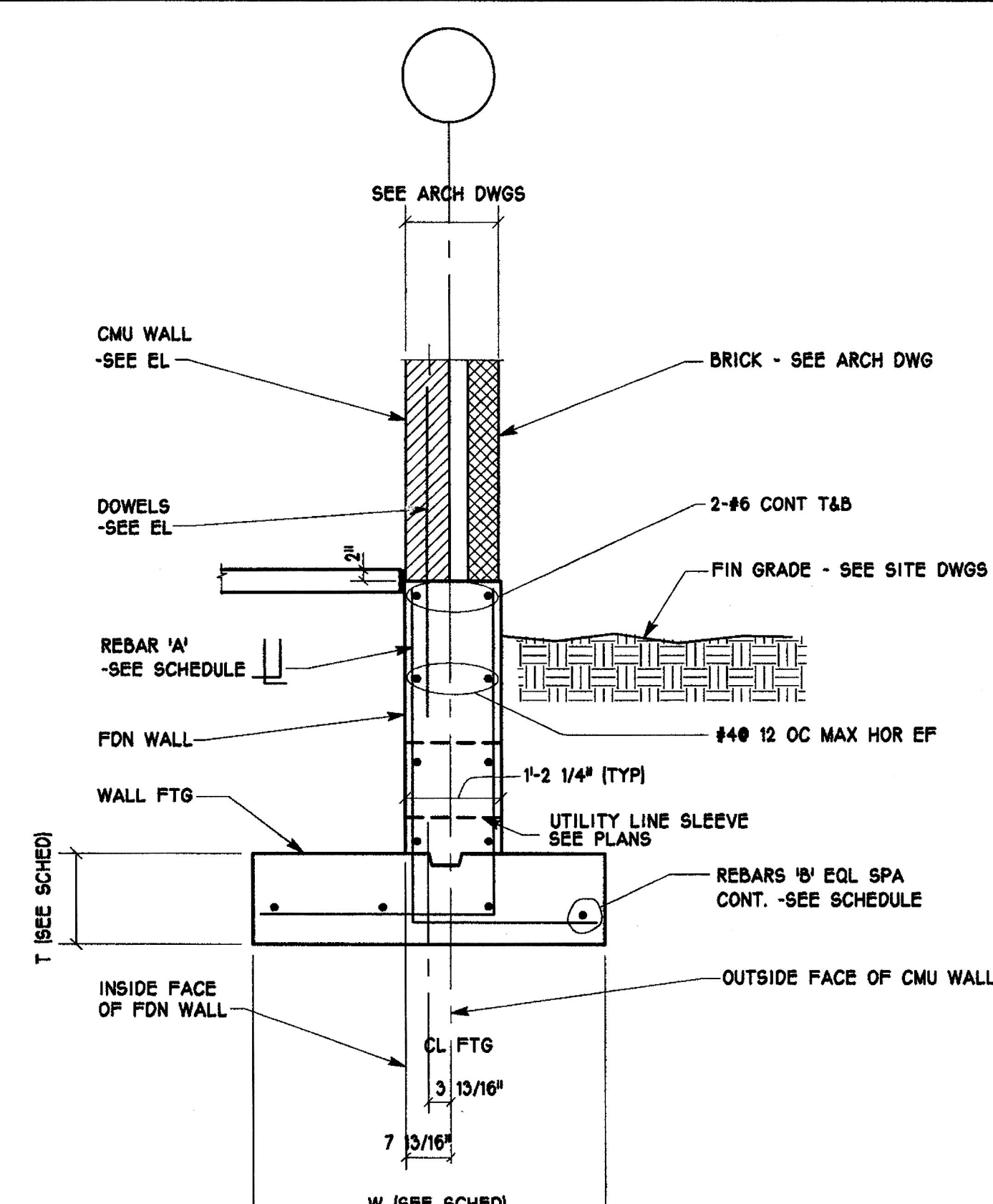
WALL FOOTING TYPE - 1 TYPICAL EXTERIOR WALL FOOTING DETAIL
