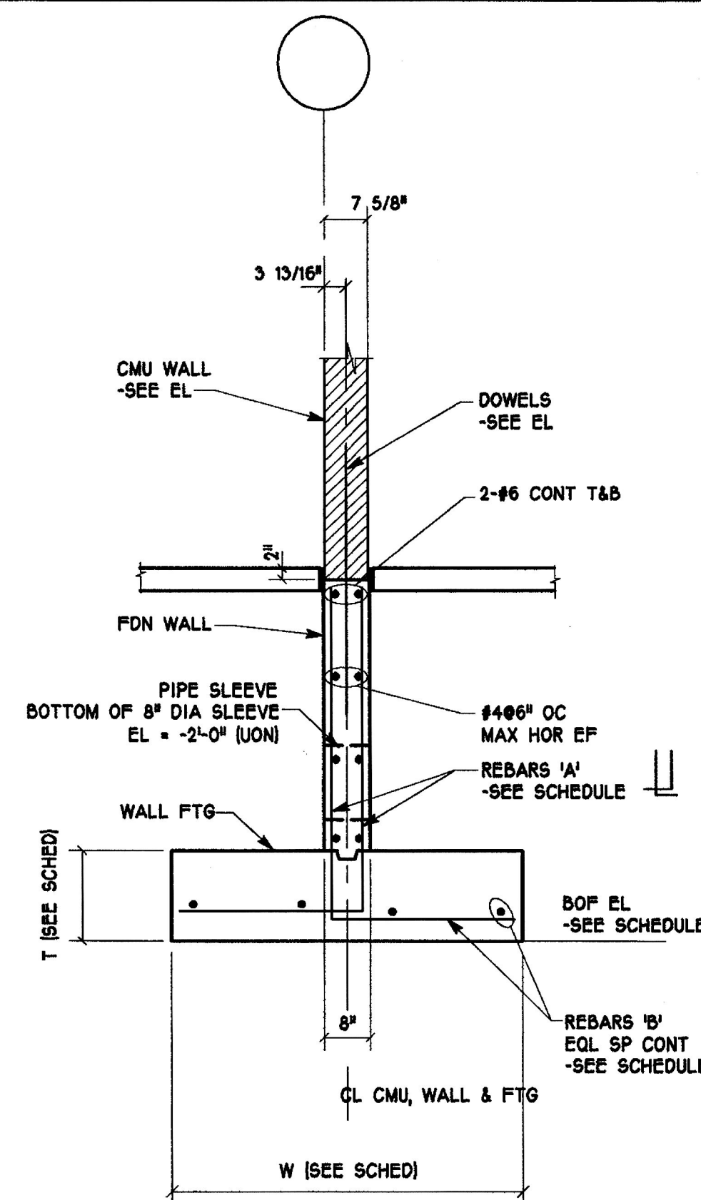
WALL FOOTING TYPE - 2 TYPICAL INTERIOR WALL FOOTING DETAIL
