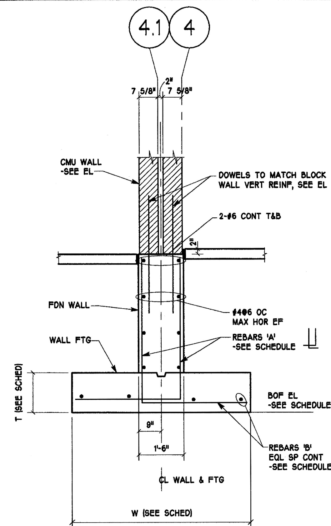
WALL FOOTING TYPE - 3 TYPICAL INTERIOR WALL FOOTING @ EXPANSION JOINT
