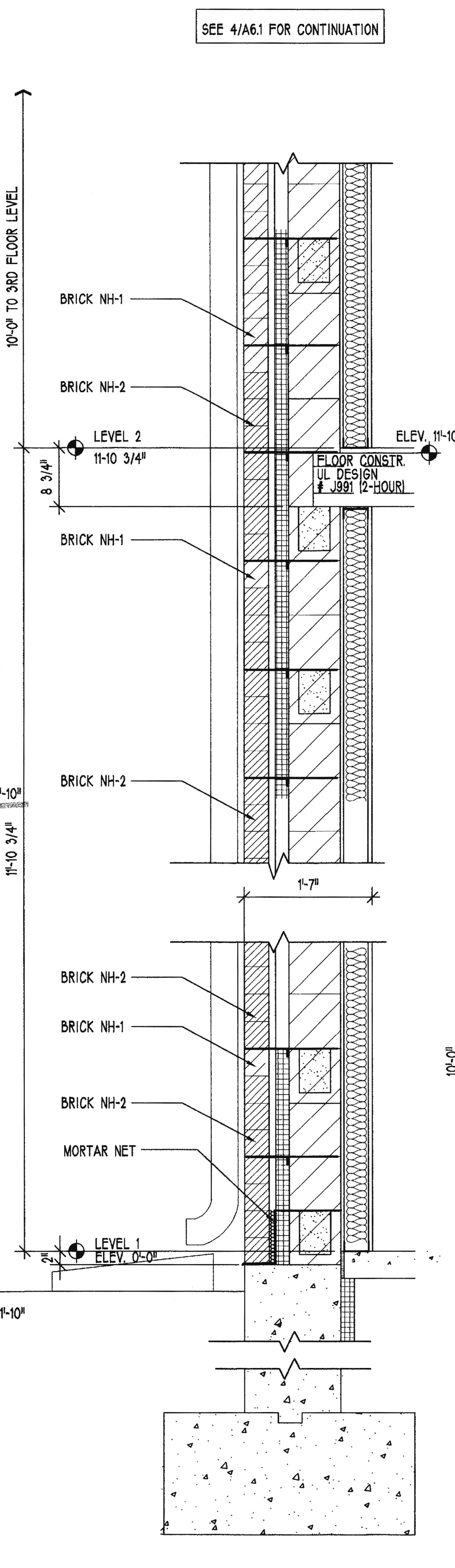
3 A6.1 TYPICAL WALL SECTION 1" = 1'
