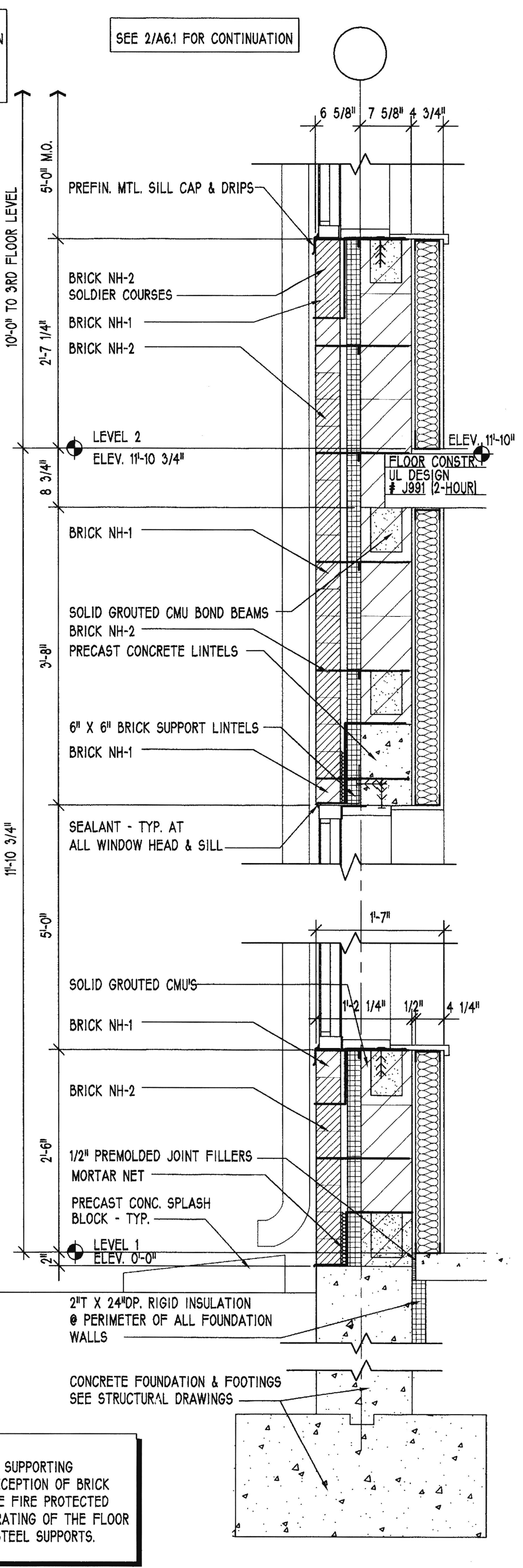
1 A6.1 P641 & P641A WALL SECTION 1" = 1'
