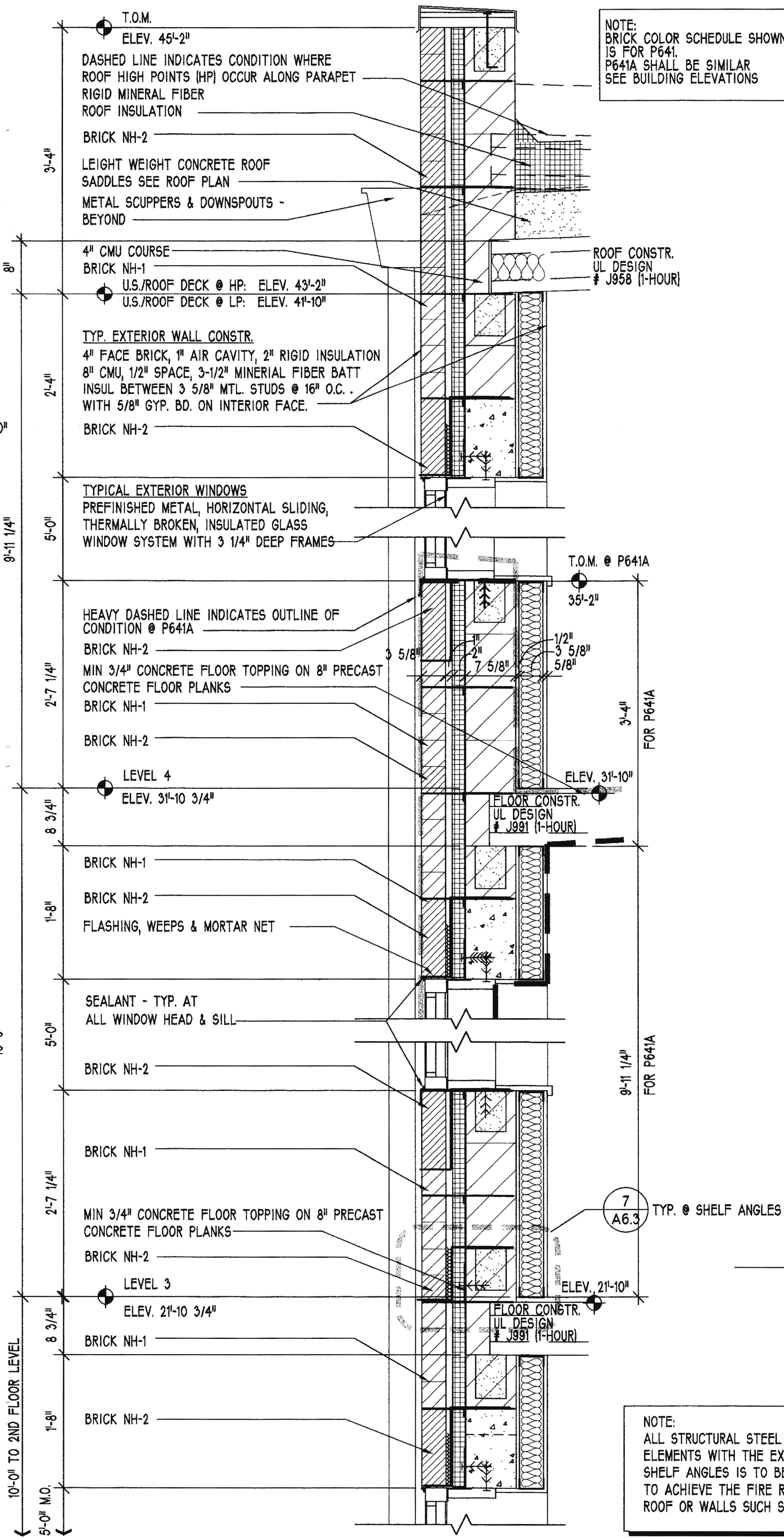
2 A6.1 P641 & P641A WALL SECTION - CONT. 1" = 1'
