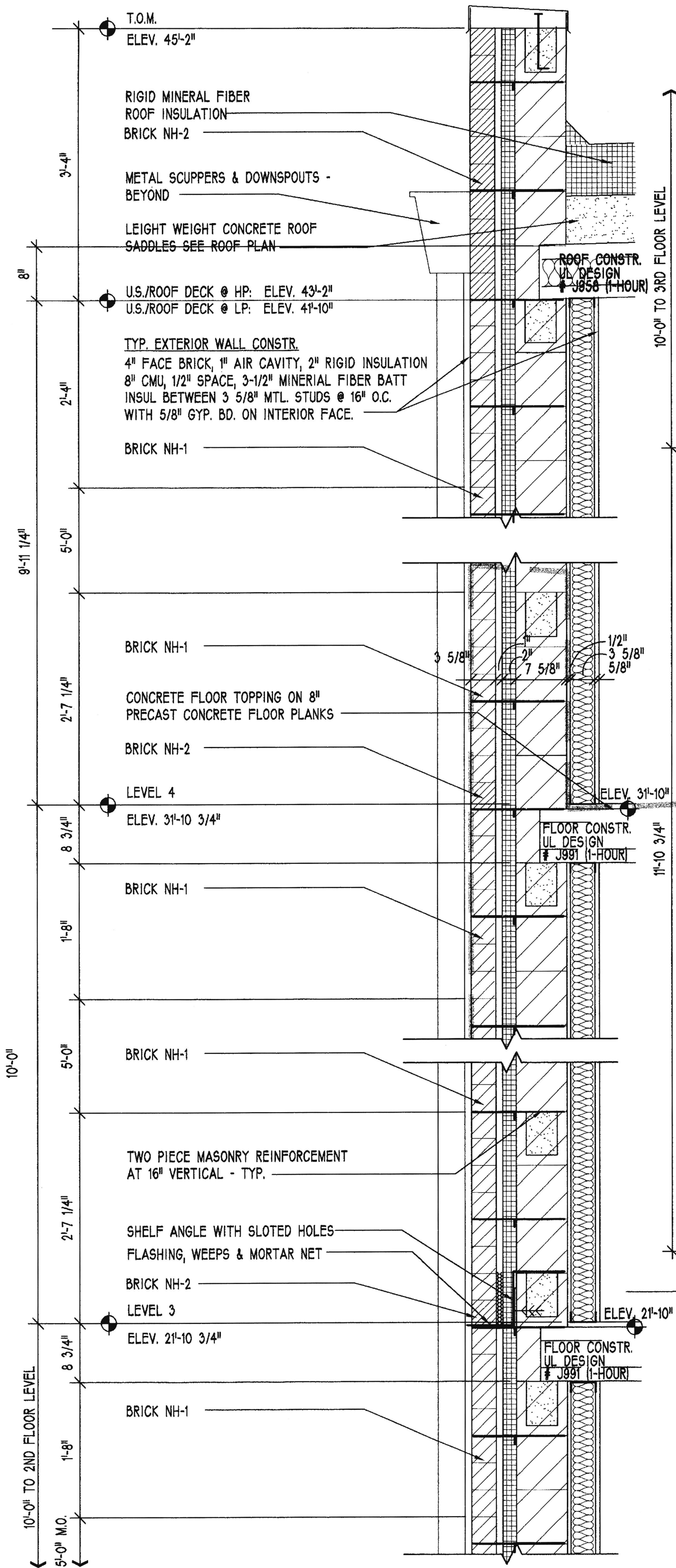
4 A6.1 TYPICAL WALL SECTION 1" = 1'
