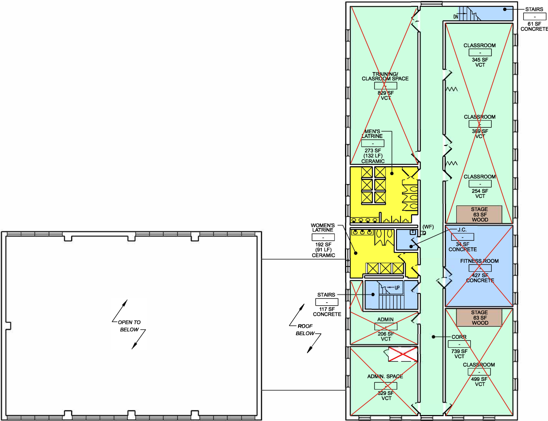
2 SECOND FLOOR CUSTODIAL SERVICE PLAN - USARC SCALE: 1/16" = 1'-0"
