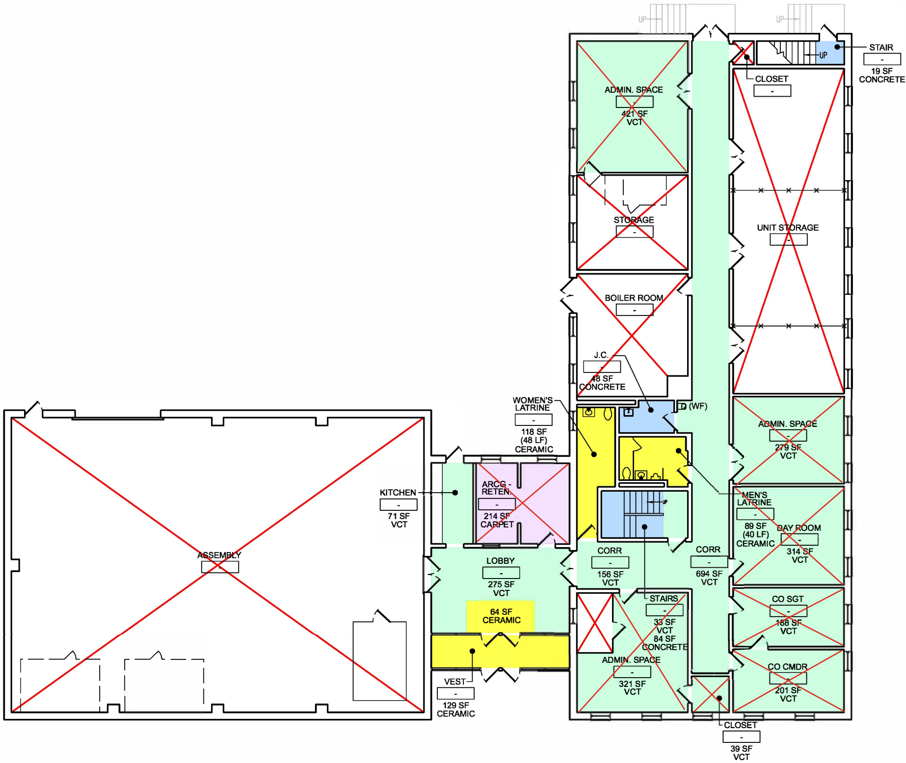
1 FIRST FLOOR CUSTODIAL SERVICE PLAN - USARC SCALE: 1/16" = 1'-0"
