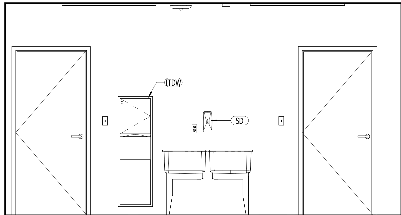
A1 ELEVATION AT FEMALE 111 - PLAN WEST SCALE: 1/2" = 1'-0"
