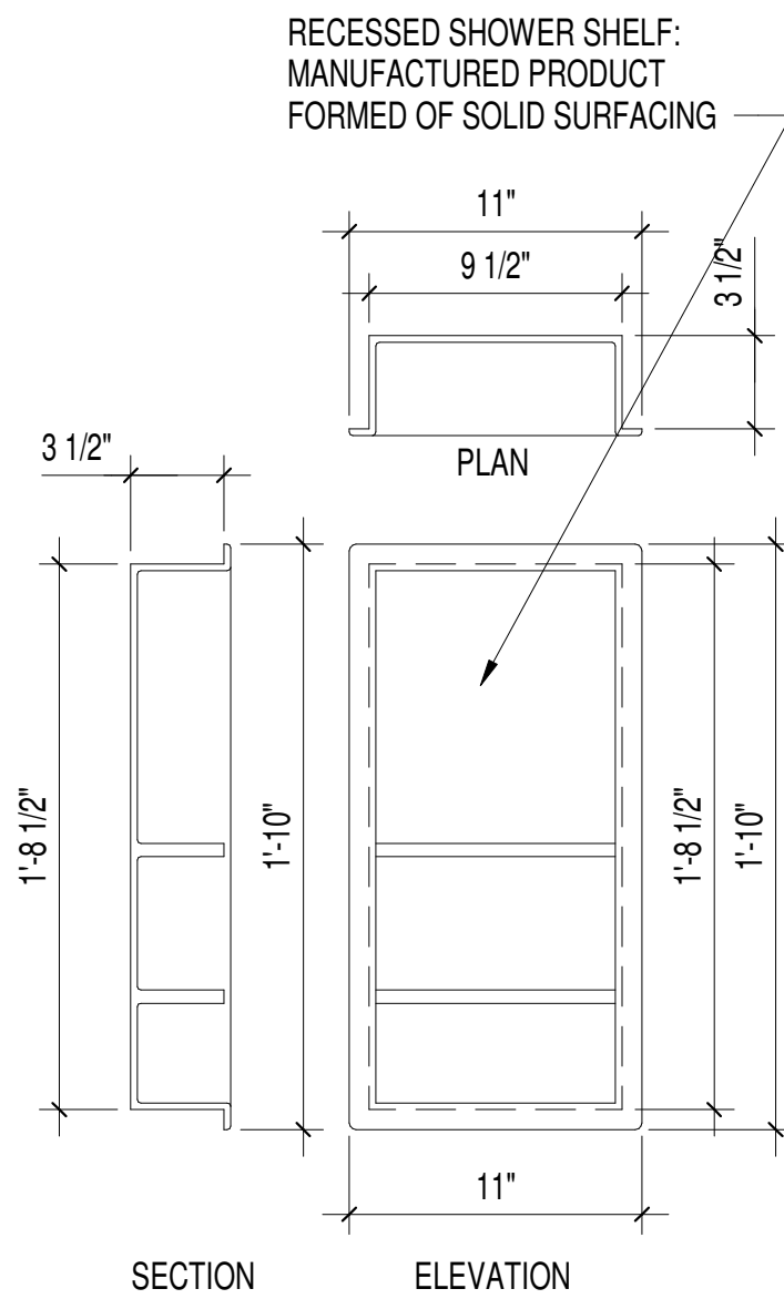
RECESSED SHOWER SHELF
