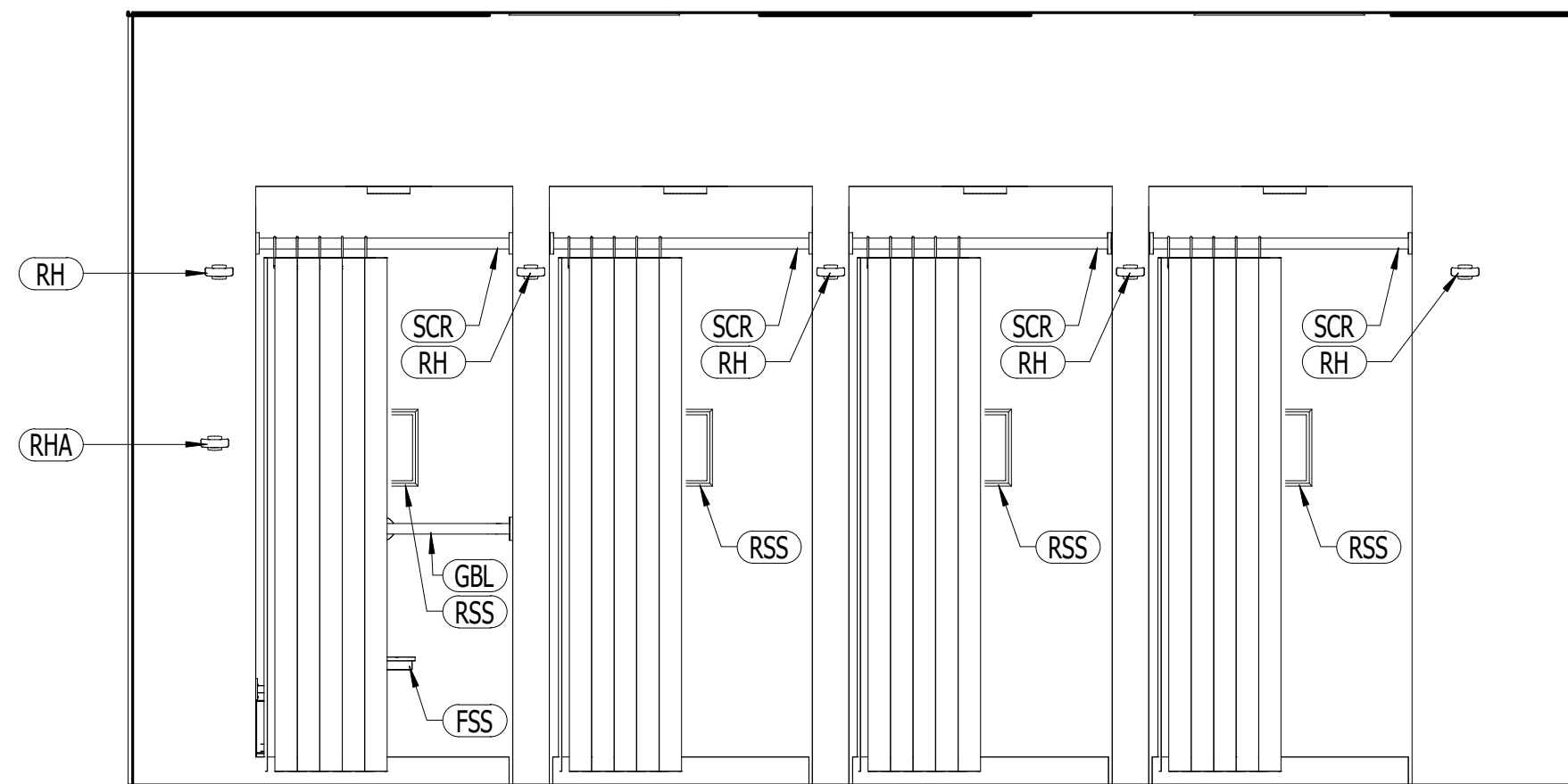
A3 ELEVATION AT FEMALE 111 - PLAN EAST SCALE: 1/2" = 1'-0"
