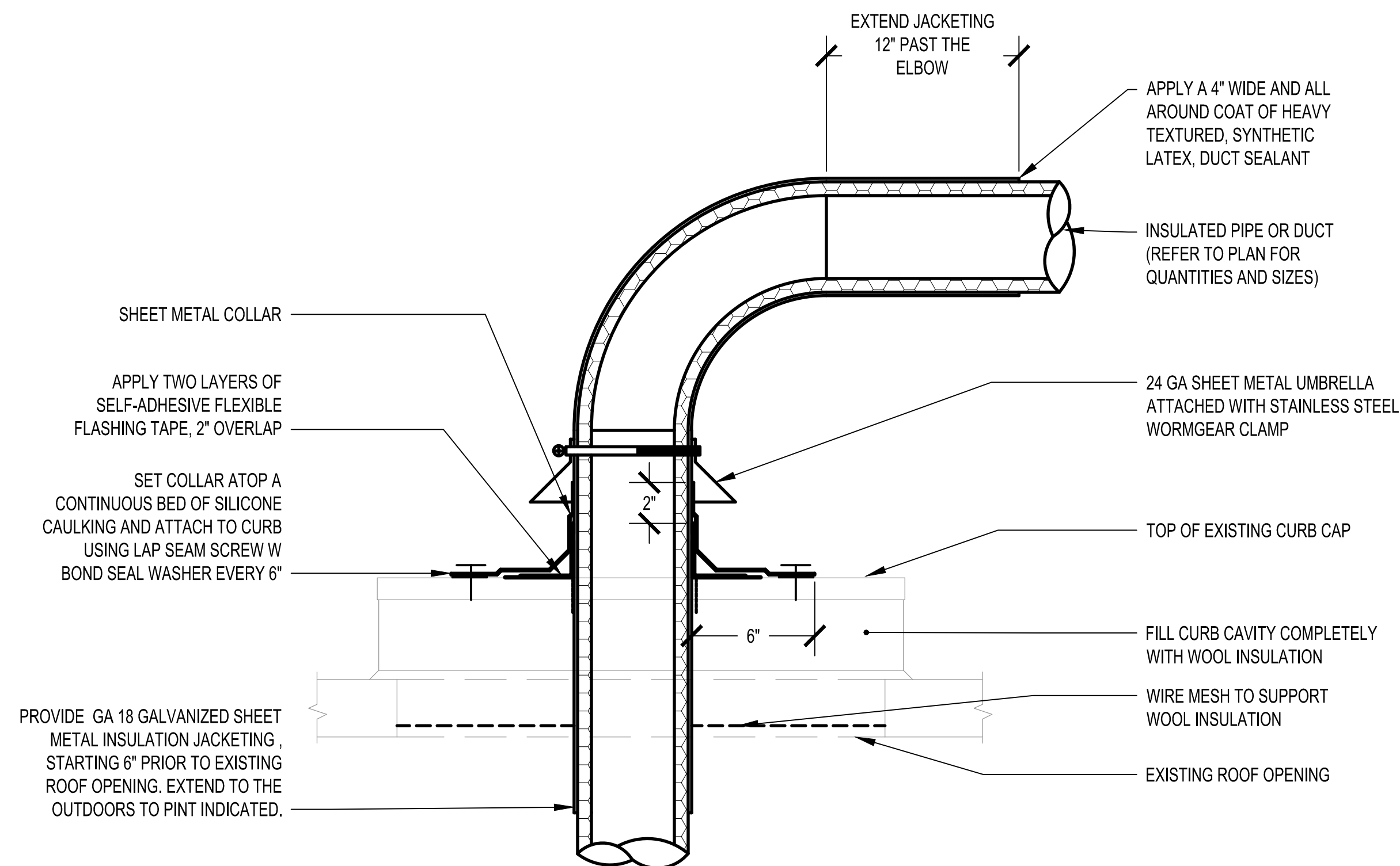
A3 DETAIL - CURB PENETRATION NOT TO SCALE
