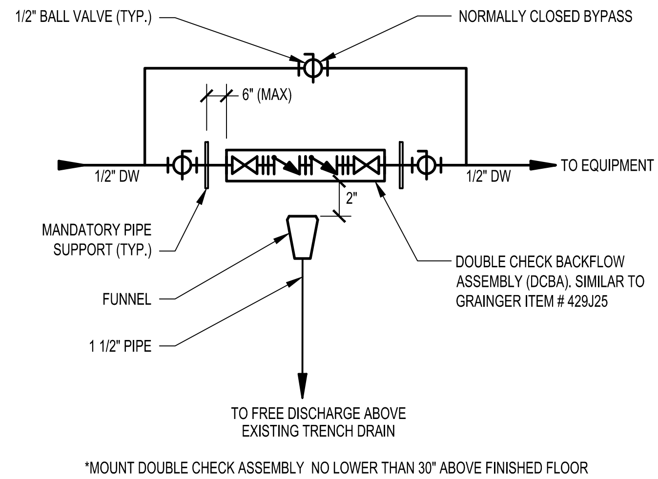
C2 DETAIL - DOUBLE BACK FLOW PREVENTER NOT TO SCALE
