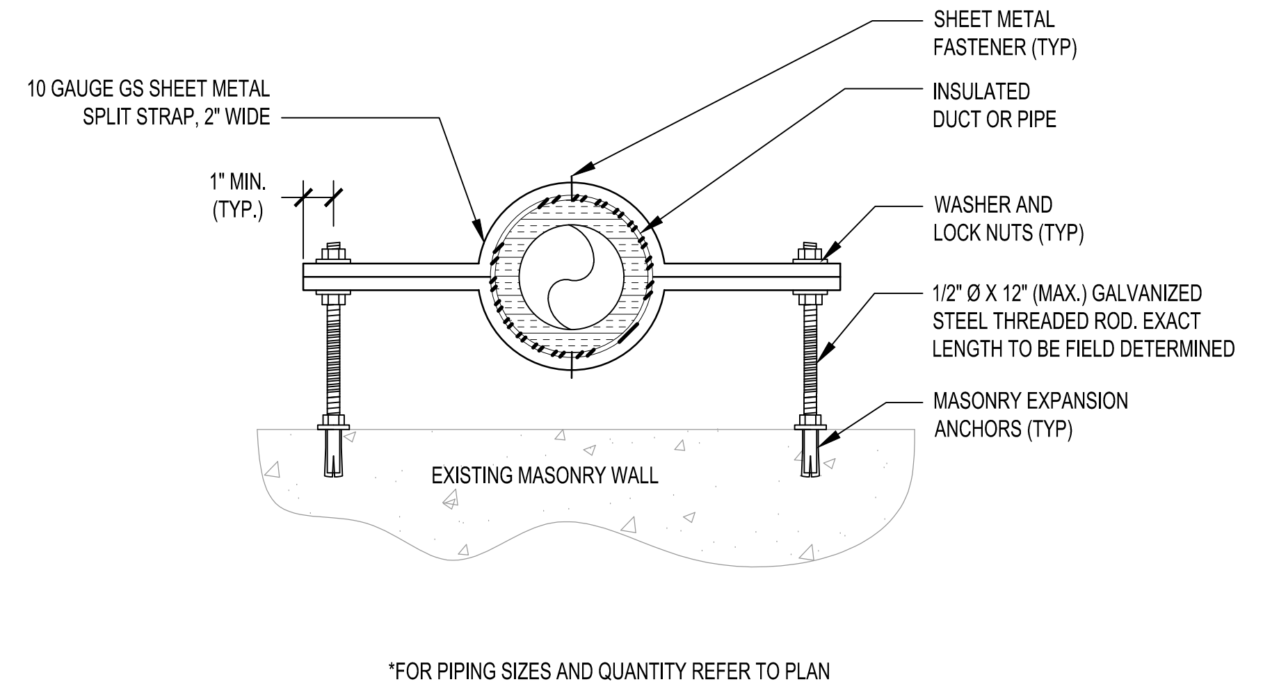
C5 DETAIL -WALL SUPPORT NOT TO SCALE
