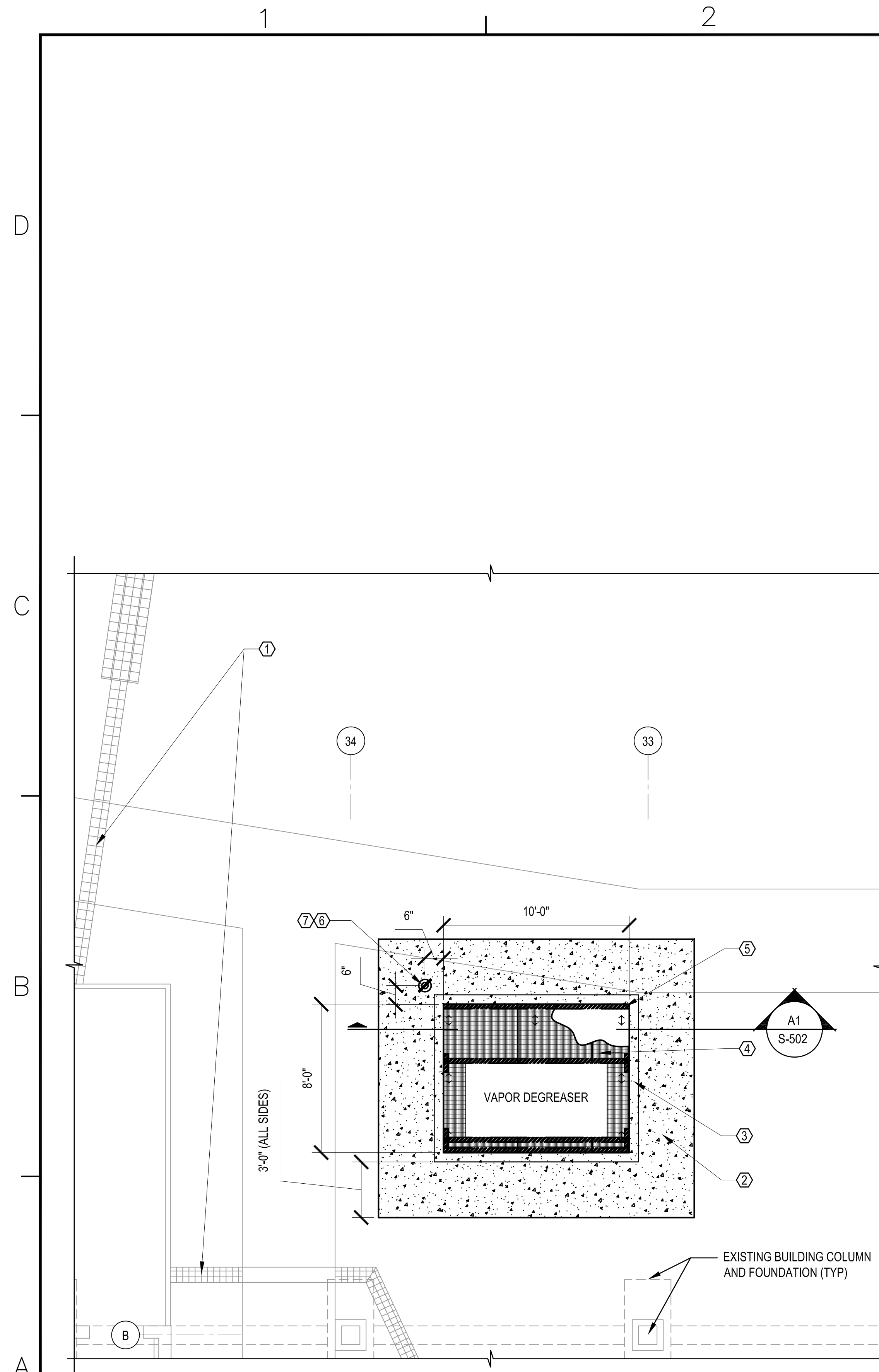
STRUCTURAL FLOOR PLAN - CONSTRUCTION
