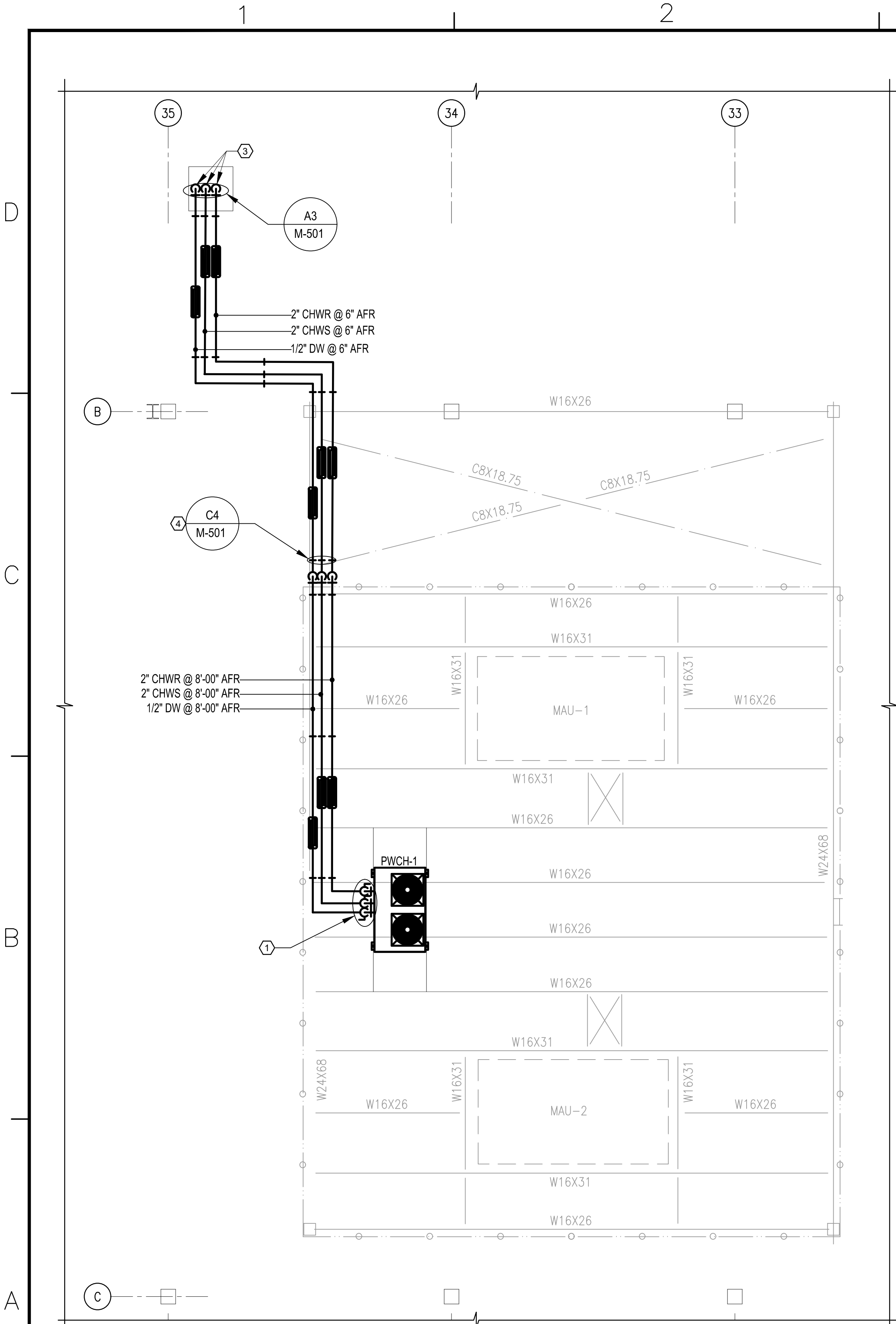
MECHANICAL ROOF PLAN - CONSTRUCTION
