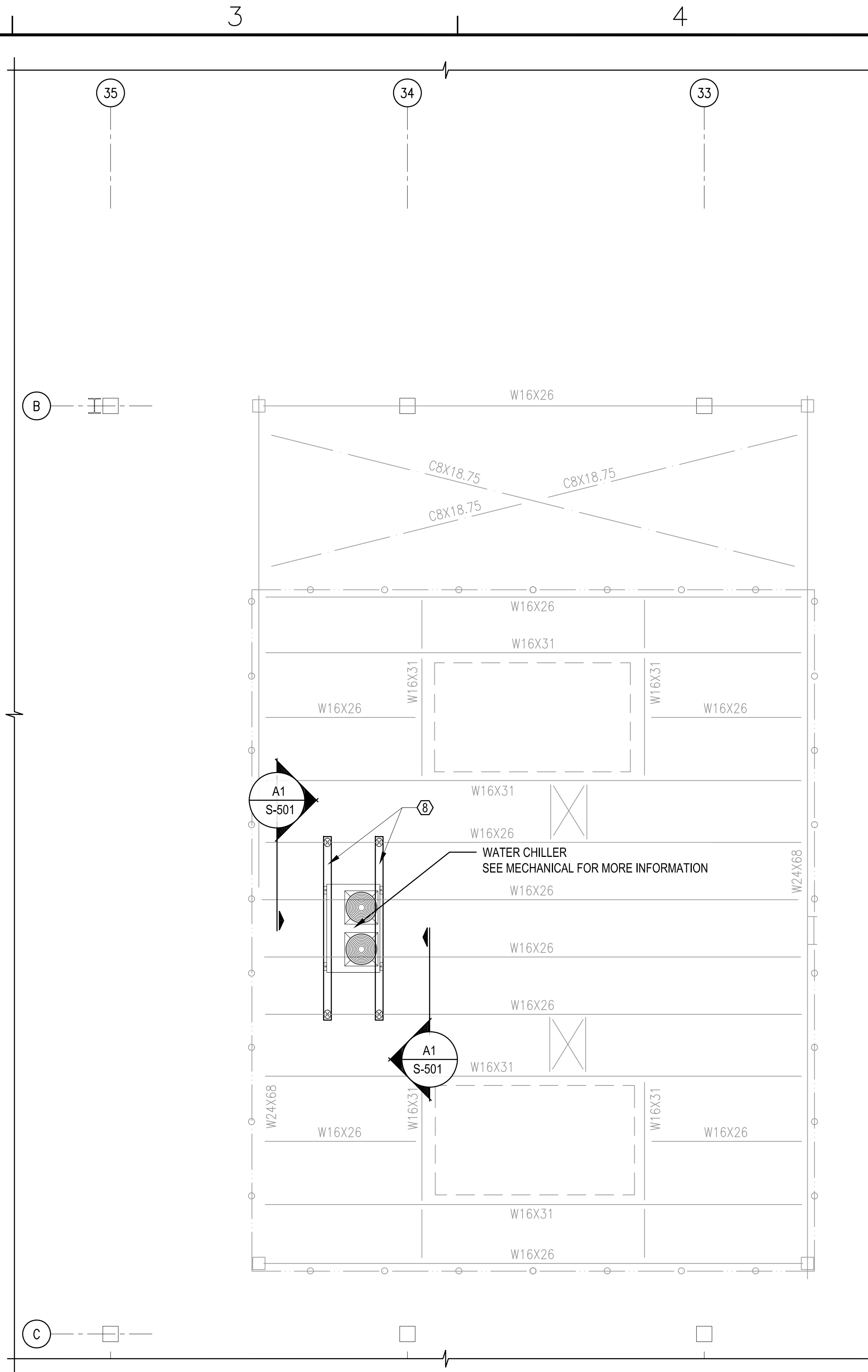
STRUCTURAL ROOF PLAN - CONSTRUCTION
