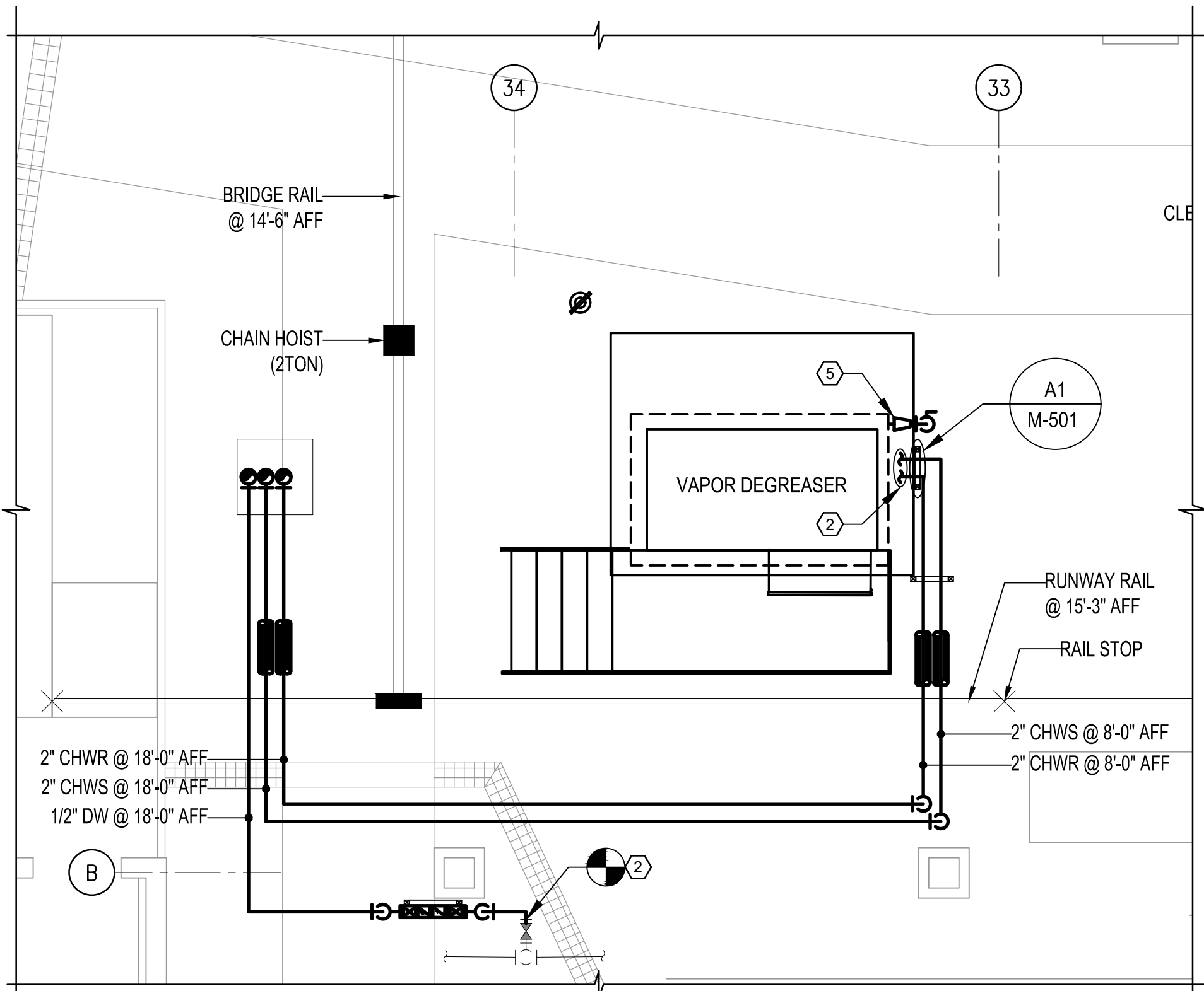
MECHANICAL FLOOR PLAN - CONSTRUCTION
