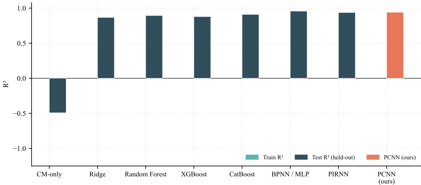
(a) Train vs Test R^2 — Overfitting Comparison
