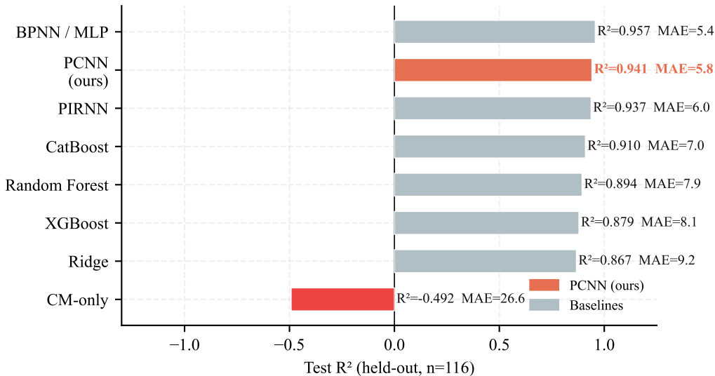
(b) Test Set Performance Ranking
