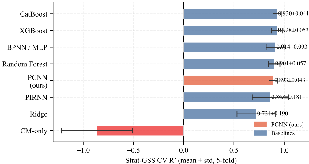
(c) Cross-Validation Stability (Strat-GSS)
