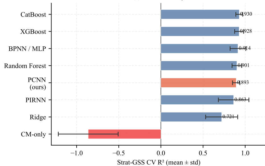
(c) CV Stability
