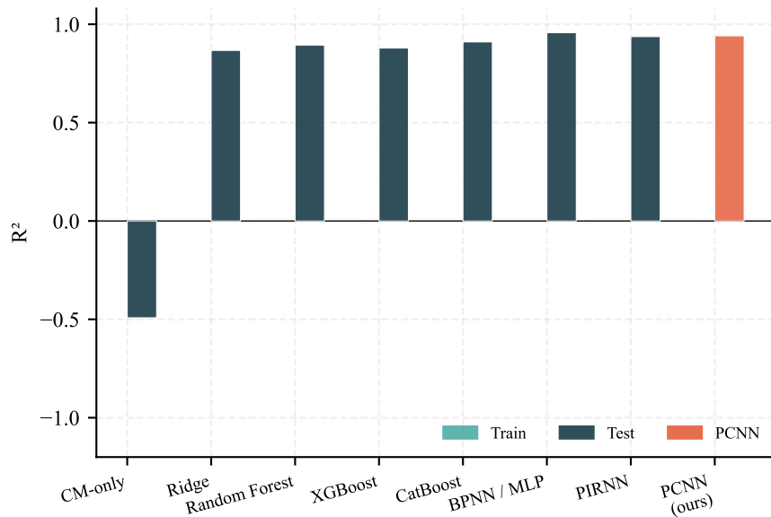
(c) CV Stability
