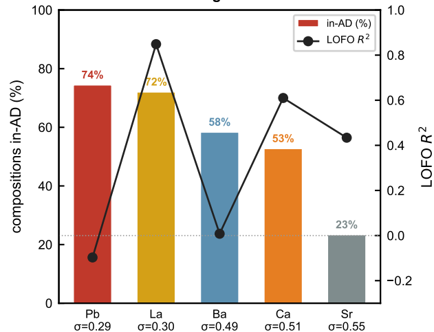
b Confident-but-wrong failure mode
