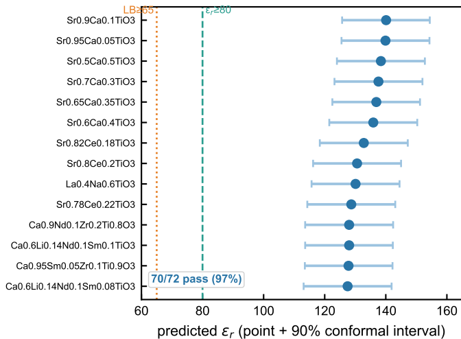
c Uncertainty-aware virtual screening
