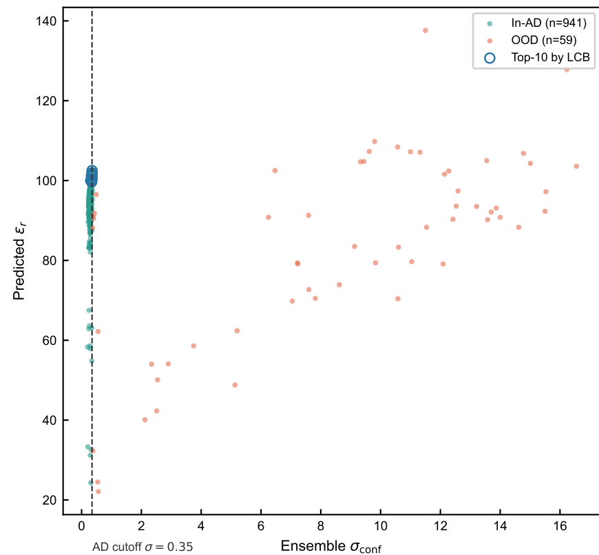
c BO-selected: \varepsilon_r vs \sigma_{conf}
