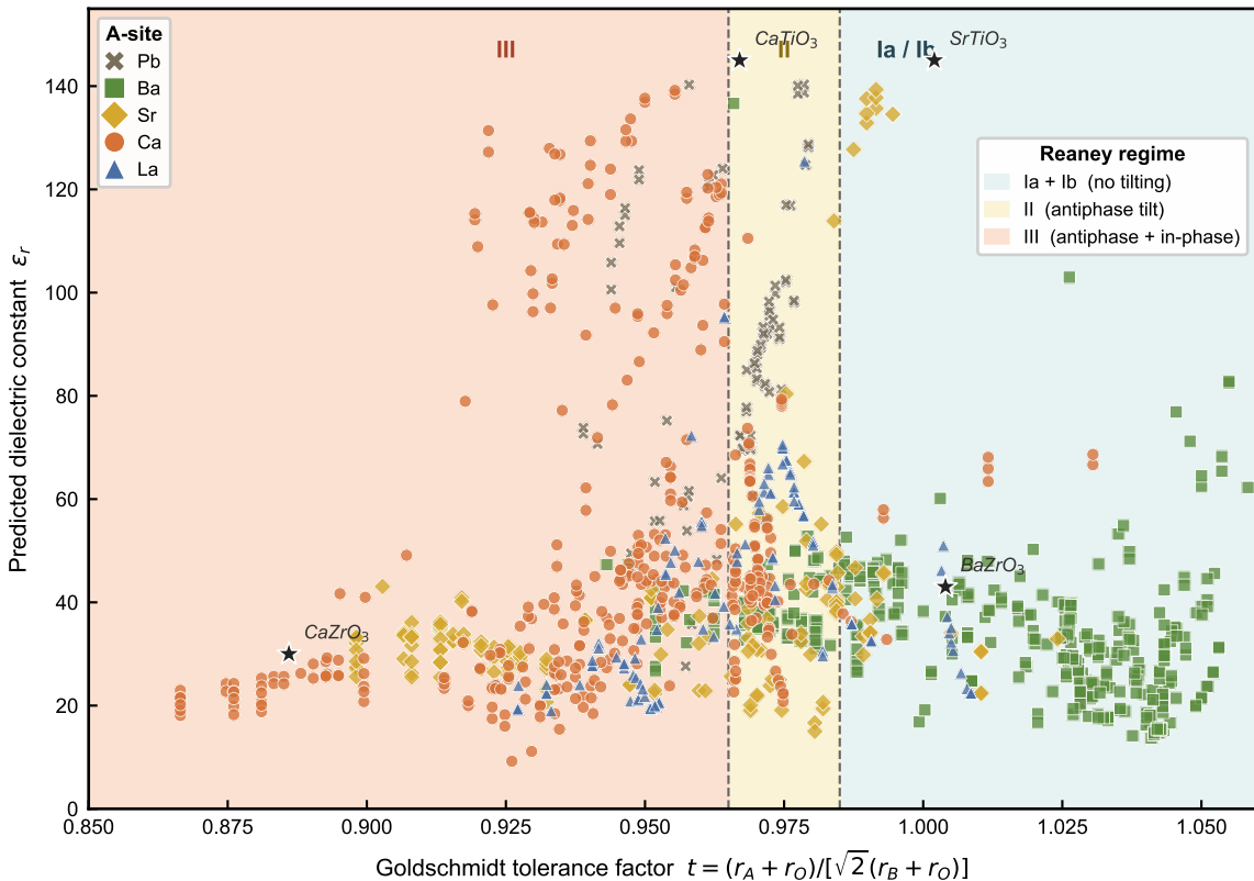
Reaney plot — PCNN predictions across the ABO 3 tolerance space
