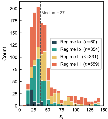
a Dataset distribution ( n=1304 )
