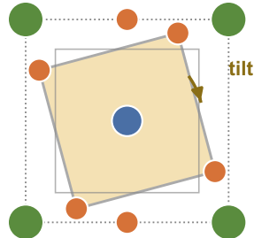
(c) Octahedral tilt \delta_{\text{tilt}} Goldschmidt/Reaney suppression
