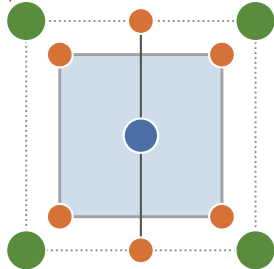
(a) Ideal cubic \text{ABO}_3 \epsilon_r^{\text{CM}} Clausius-Mossotti baseline
