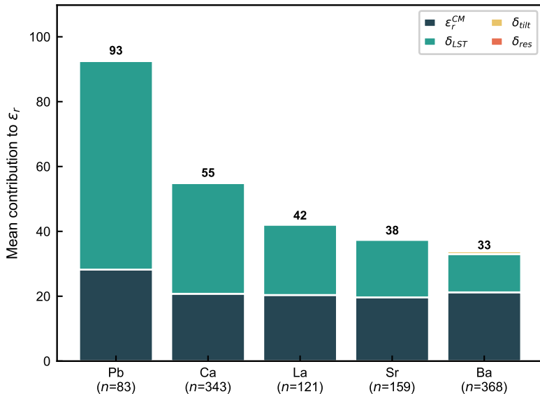
a Per-A-site decomposition
