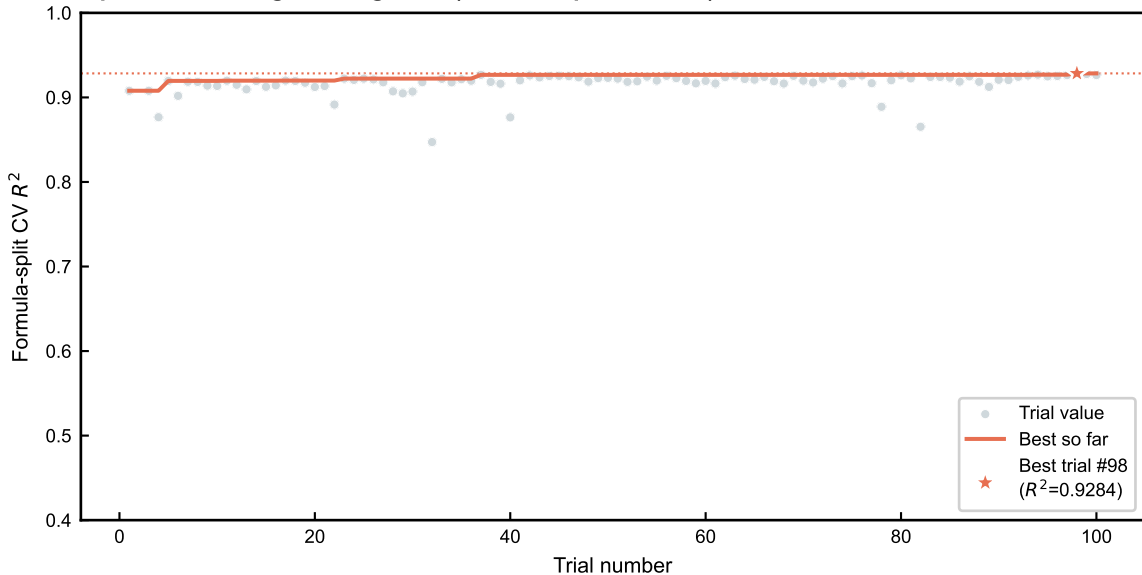
Optuna HP tuning convergence ( n=99 completed trials)
