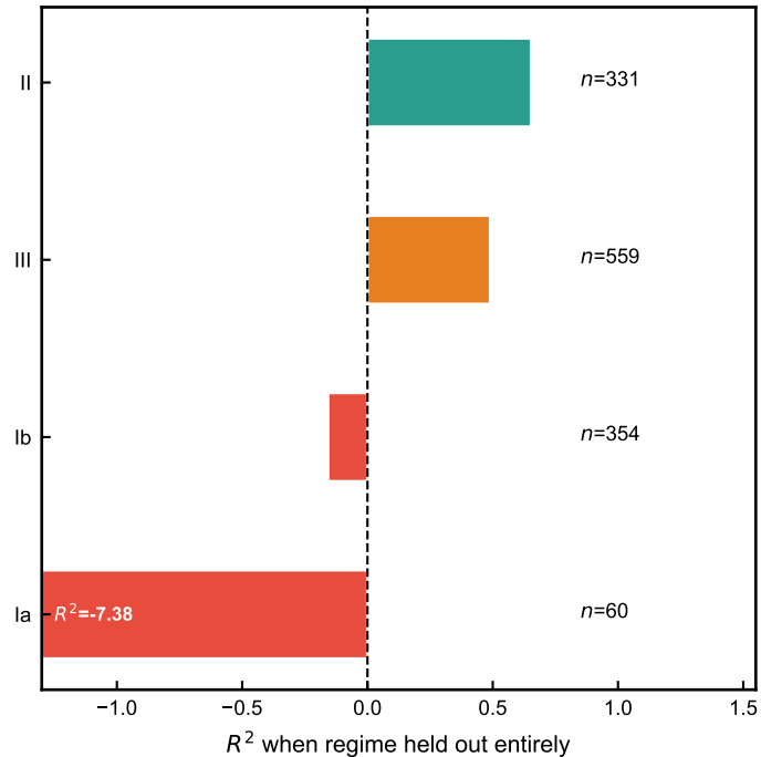
b Leave-one-family-out: Reaney regime
