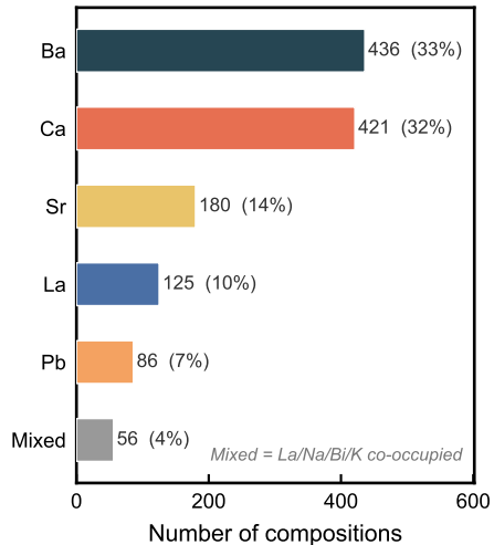
c A-site occupancy
