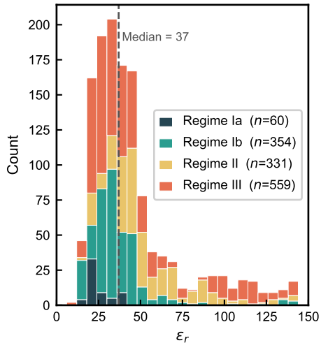
a Dataset distribution ( n=1304 )
