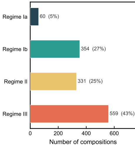
b Reaney regime distribution
