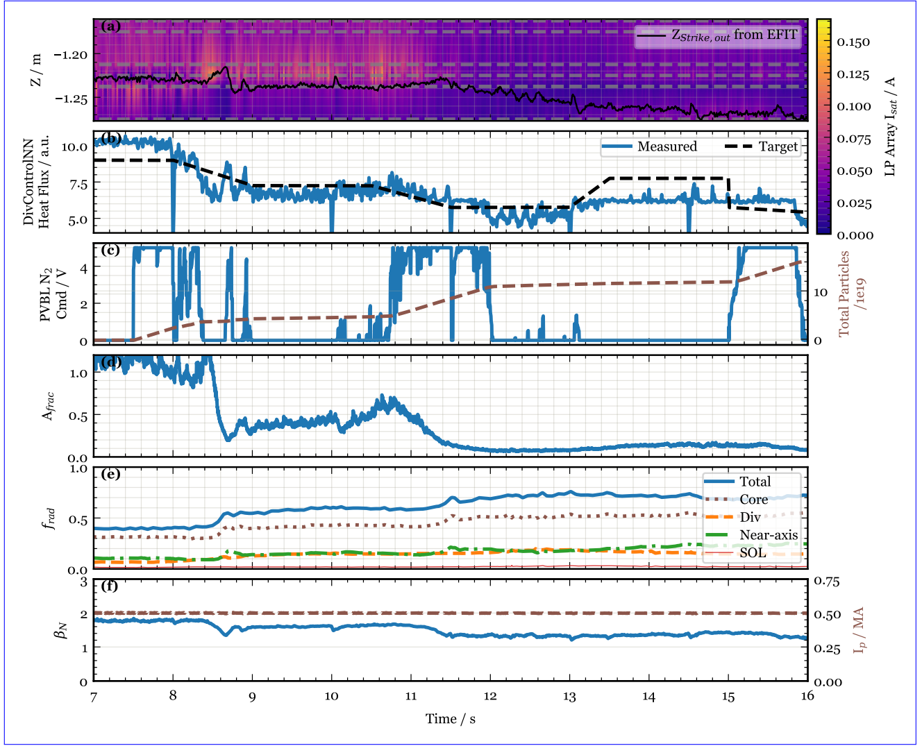
Figure 9. Detachment control shot #36161 using DivControlNN heat flux at outer divertor. (a) Shows the measured ion saturation current by realtime Langmuir-Probe -LP array at locations marked by grey dashed lines. The data has been interpolated spatially using cubic spline interpolation. The black curve shows the post-shot calculated strike point position on outer divertor using EFIT. (b) Shows the heat flux at outer divertor calculated by DivControlNN. The dashed black line shows the target provided to the controller to follow. (c) Left axis: Shows the N 2 gas command steps sent for system identification. Right axis: Shows the cumulative N 2 gas particles injected into the vessel. (d) Left axis: Shows the A_{frac} calculated from peak value among the Langmuir probe -LP array. Right axis: Total radiated power measured by Infra-Red Video Bolometer (IRVB). (e) Left axis: Shows \beta_n . Right axis: Shows the plasma current ( I_p ).
