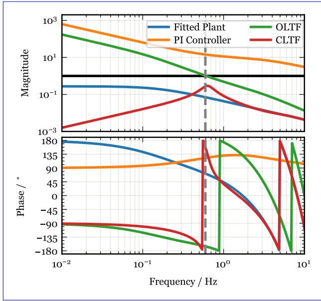
Figure 4. Closed loop transfer function analysis of the system using A_{frac}A_{frac} output with chosen PI controller with gains: K_p = -10.0 , T_i = 253.0 ms, and \tau_s = 50.0 ms. The dashed grey vertical line shows the unity gain frequency (UGF) of the system.
