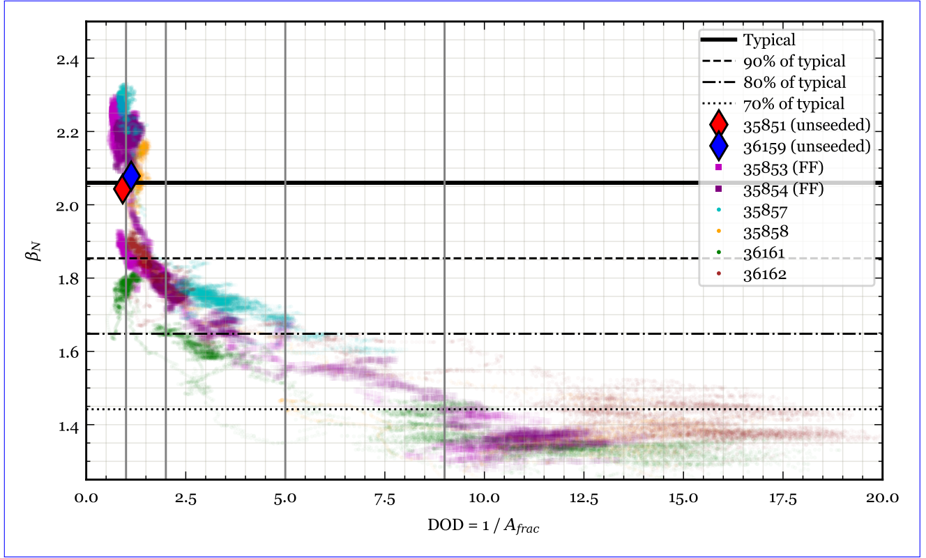
Figure 13. Normalized \beta_N plotted versus degree of detachment DOD = 1/A_{frac} . A_{frac} has been renormalized so that all shots have the same empirical correction factor. For seeded shots, the time range is from t = 6.0 s until I_p begins to drop. For unseeded shots, values are averaged over 6.0 < t < 8.0 s. Vertical lines are placed as guides at DOD = 1, 2, 5 , and 9 , corresponding to guides and the axis limit of figure 12 of [21]. Horizontal black lines mark typical \beta_N values of attached shots in this scenario as well as various levels of degradation (see legend). Unseeded shots are marked by opaque diamonds giving their average values over a period of steady performance during the I_p flattop.
