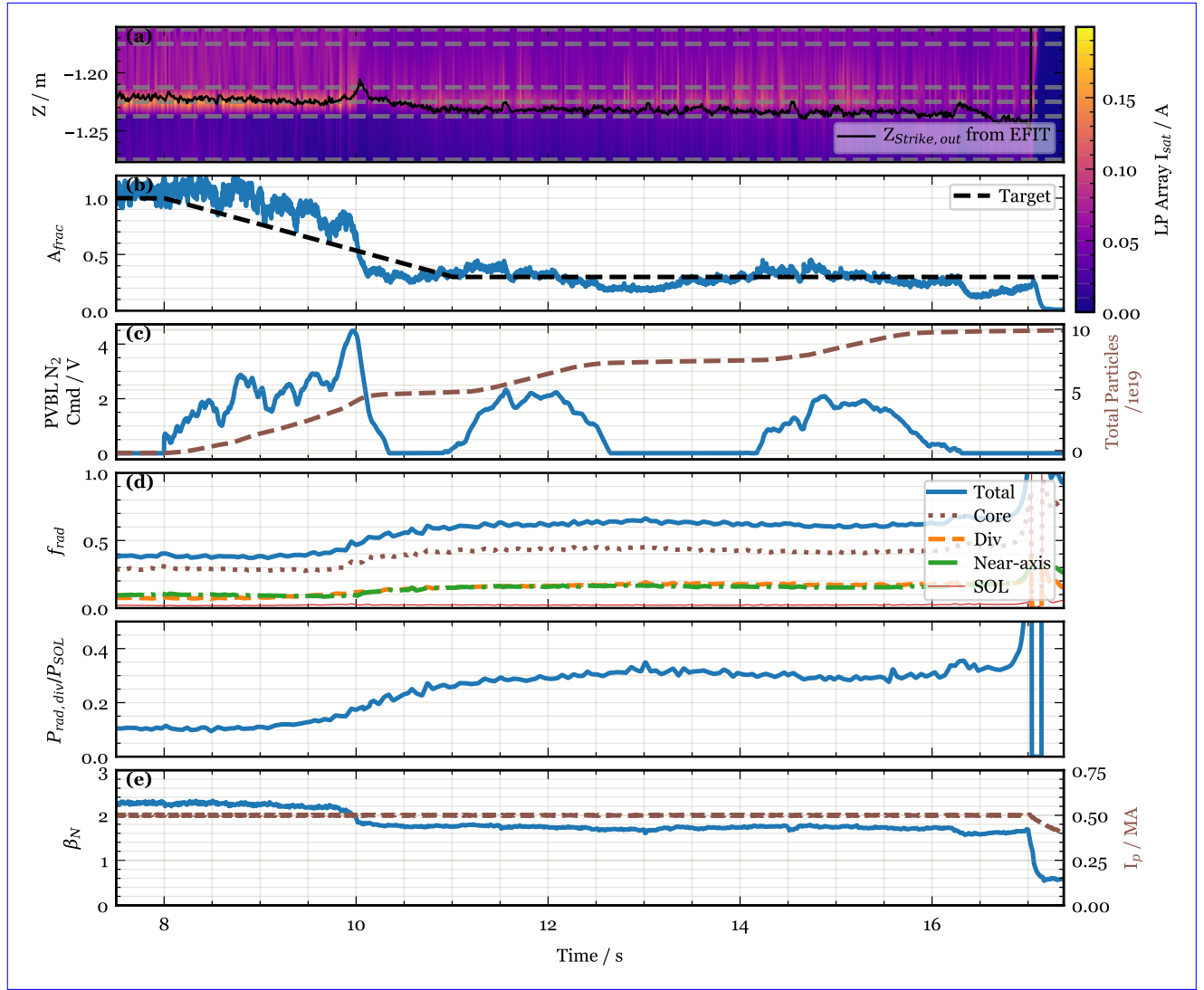
Figure 8. Detachment control shot #35857 using A_{frac} controller. (a) Shows the measured ion saturation current by realtime Langmuir Probe -LP array at locations marked by grey dashed lines. The data has been interpolated spatially using cubic spline interpolation. The black curve shows the post-shot calculated strike point position on outer divertor using EFIT. (b) Shows the A_{frac} calculated from peak value among the Langmuir probe -LP array. The dashed black line shows the target provided to the controller to follow. (c) Left axis: Shows the N_2 gas command steps sent for system identification. Right axis: Shows the cumulative N_2 gas particles injected into the vessel. (d) Total radiated power measured by Infra-Red Video Bolometer (IRVB). (e) Left axis: Shows \beta_N . Right axis: Shows the plasma current ( I_p ). One of the EC sources stops at 16.2 s, causing a drop in \beta_N (e) and A_{frac} (b).
