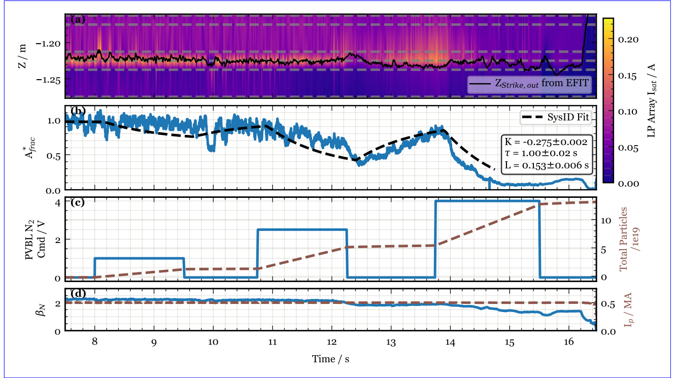
Figure 3. System identification shot #35853. (a) Shows the measured ion saturation current by realtime Langmuir Probe Langmuir probe (LP) array at locations marked by grey dashed lines. The data has been interpolated spatially using cubic spline interpolation. The black curve shows the post-shot calculated strike point position on outer divertor using EFIT. (b) Shows the A_{frac} calculated from peak value among the Langmuir probe Langmuir probe (LP) array. The dashed black line shows the system identification fit on this data. (c) Left axis: Shows the N_2 gas command steps sent for system identification. Right axis: Shows the cumulative N_2 gas particles injected into the vessel. (d) Left axis: Shows \beta_n . Right axis: Shows the plasma current ( I_p ). * Note: A_{frac} for this shot was not calibrated properly and the raw data reported 2 times the value. We fixed this factor after this shot and this figure shows the corrected value.
