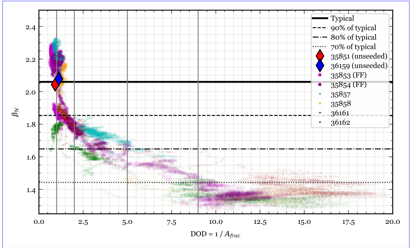
Figure 13. Normalized \beta plotted versus degree of detachment DOD = 1/A_{frac} . A_{frac} has been renormalized so that all shots have the same empirical correction factor. For seeded shots, the time range is from t = 6.0 s until I_p begins to drop. For unseeded shots, values are averaged over 6.0 < t < 8.0 s. Vertical lines are placed as guides at DOD = 1, 2, 5 , and 9 , corresponding to guides and the axis limit of figure 12 of [21]. Horizontal black lines mark typical \beta_N values of attached shots in this scenario as well as various levels of degradation (see legend). Unseeded shots are marked by opaque diamonds giving their average values over a period of steady performance during the I_p flattop.
