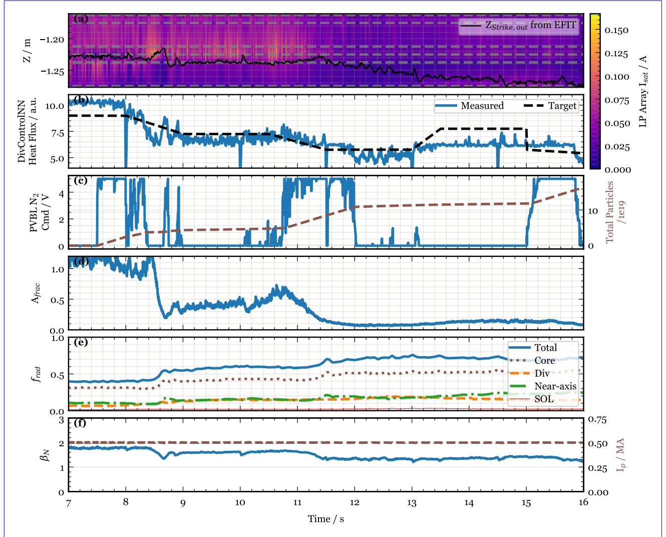
Figure 9. Detachment-control Control shot #36161 using DivControlNN heat flux at outer divertor. (a) Shows the measured ion saturation current by realtime Langmuir Probe -LP array at locations marked by grey dashed lines. The data has been interpolated spatially using cubic spline interpolation. The black curve shows the post-shot calculated strike point position on outer divertor using EFIT. (b) Shows the heat flux at outer divertor calculated by DivControlNN. The dashed black line shows the target provided to the controller to follow. (c) Left axis: Shows the N 2 gas command steps sent for system identification. Right axis: Shows the cumulative N 2 gas particles injected into the vessel. (d) Left axis: Shows the A_{frac} calculated from peak value among the Langmuir probe -LP array. Right axis: Total radiated power measured by Infra-Red Video Bolometer (IRVB). (e) Left axis: Shows \beta_n . Right axis: Shows the plasma current ( I_p ).
