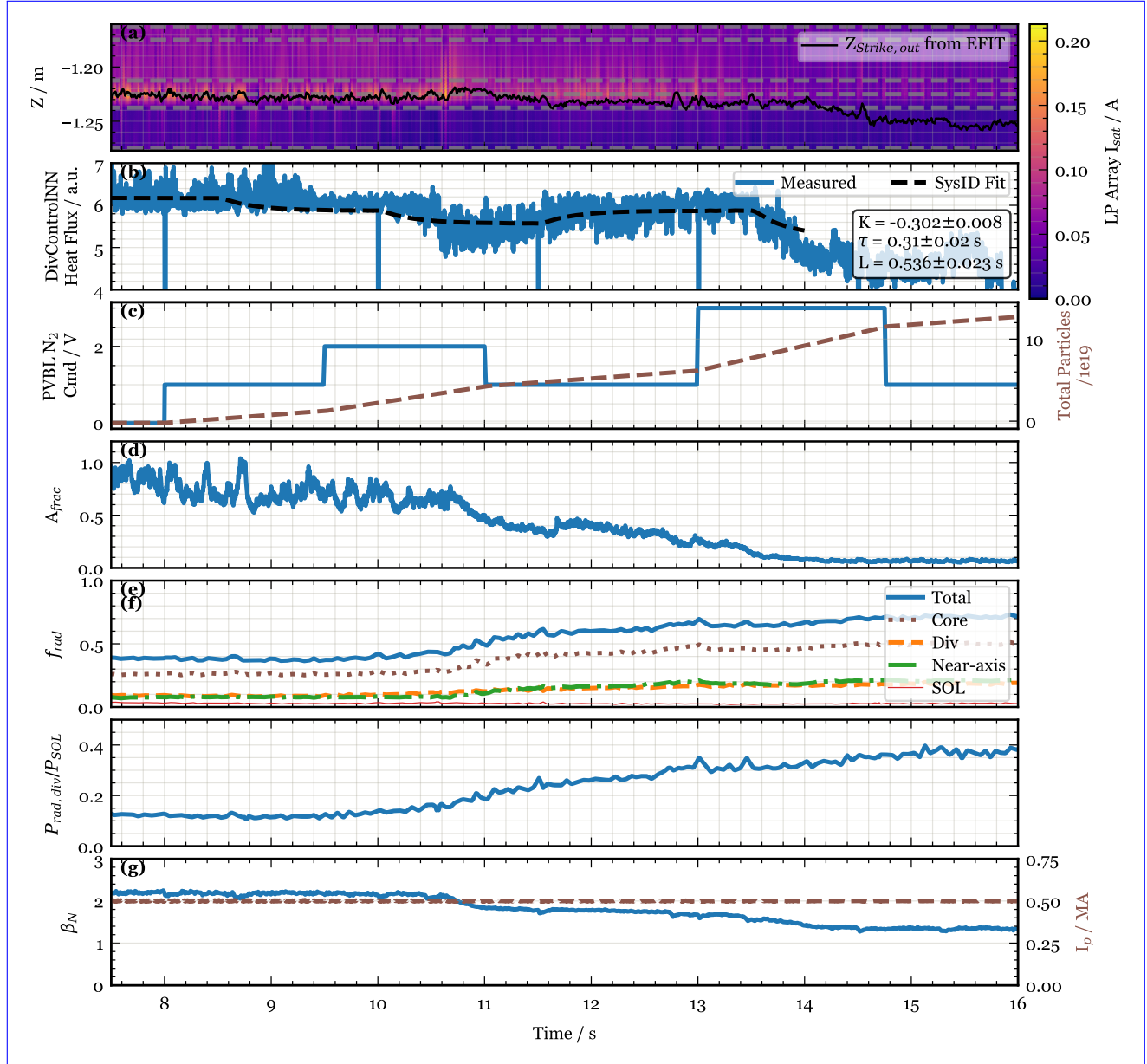
Figure 5. System identification shot #35854. (a) Shows the measured ion saturation current by realtime Langmuir-Probe -Langmuir probe (LP) array at locations marked by grey dashed lines. The data has been interpolated spatially using cubic spline interpolation. The black curve shows the post-shot calculated strike point position on outer divertor using EFIT. (b) Shows the heat flux at outer divertor calculated by DivControlNN. The dashed black line shows the system identification fit on this data. (c) Left axis: Shows the N_2 gas command steps sent for system identification. Right axis: Shows the cumulative N_2 gas particles injected into the vessel. (d) Shows the A_{frac} calculated from peak value among the Langmuir-probe -Langmuir probe (LP) array. (e) Shows radiated power fraction from various zones of the plasma. (f) Left axis: Shows \beta_n . Right axis: Shows the plasma current ( I_p ).
