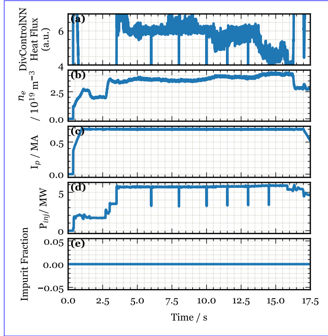
Figure 6. KSTAR #35854 DivControlNN quantities. (a) Shows the calculated heat flux at outer divertor calculated by DivControlNN. Rest of the panels are inputs to DivControlNN. (b) Shows the line averaged electron density. (c) Shows the plasma current. (d) Shows the total injected power. (e) Shows the impurity fraction estimate. Note that this calculation malfunctioned and fed constant zero input to the model even though N_2 was puffed in this shot. Apart from these inputs, diffusion scaling factor was set to a constant value of 1.0 in the model.
