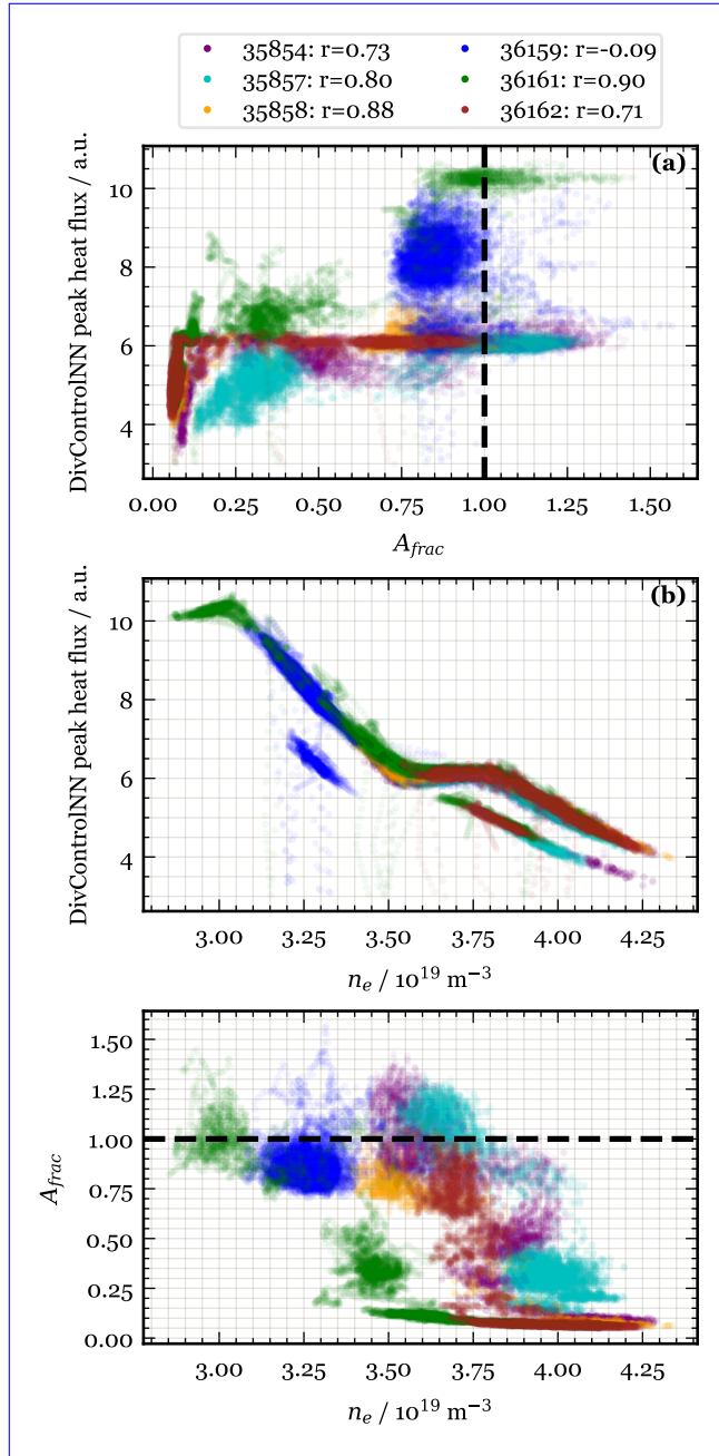
Figure 12. DivControlNN heat flux versus A_{frac} (a) and n_e (b). A_{frac} has been renormalized to use the same correction coefficient in all cases. The top legend gives Pearson r values for each shot individually. When all the data shown in panel (a) are aggregated, they have r = 0.62 . Times are from 6.2 s to the end of each shot. #35854 was a feedforward system ID shot and #36159 was unseeded; the others used detachment control.
