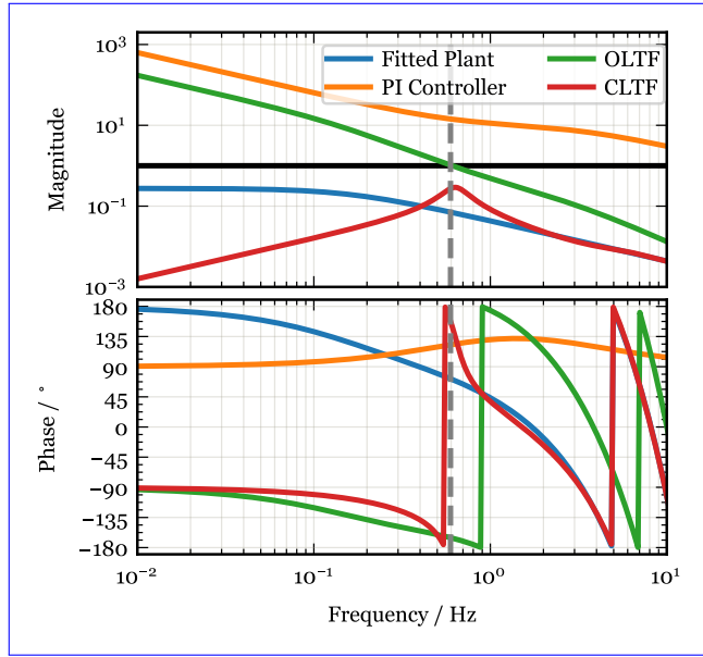
Figure 4. Closed loop transfer function analysis of the system using A_{frac} output with chosen PI controller with gains: K_p = -10.0 , T_i = 253.0 ms, and \tau_s = 50.0 ms. The dashed grey vertical line shows the unity gain frequency (UGF) of the system.
