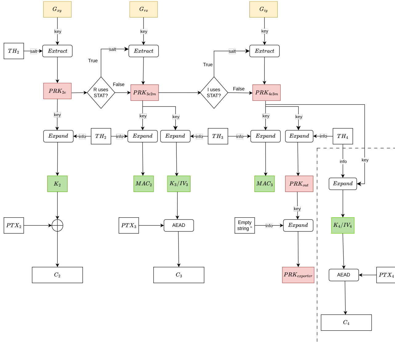
Figure 3: EDHOC key schedule. The yellow boxes denote DH-shared secrets ( G_{xy} , G_{rx} , G_{iy} ). The red boxes denote the intermediate keys ( PRK_{2e} , PRK_{3e2m} , PRK_{4e3m} , PRK_{out} , PRK_{exporter} ) and the green boxes denote MAC, encryption keys, and initial vectors ( MAC_2 , MAC_3 , K_2 , K_3/IV_3 , K_4/IV_4 ). The operations which are within the dashed area are optional and only executed if the Message 4 ( Msg_4 ) is sent to Initiator. Adapted from [Pér+24].
