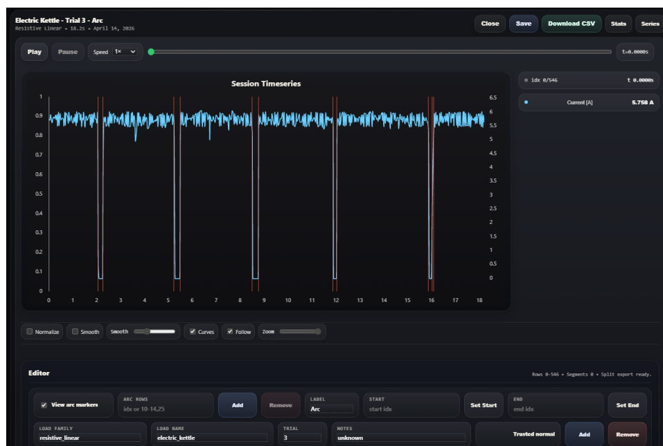
Figure 3.17. Arc labeling using logged waveform data.
