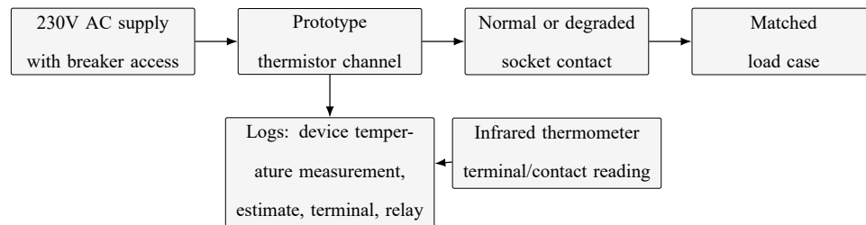
Figure 3.27. Testing setup block diagram for socket-heating evaluation.
