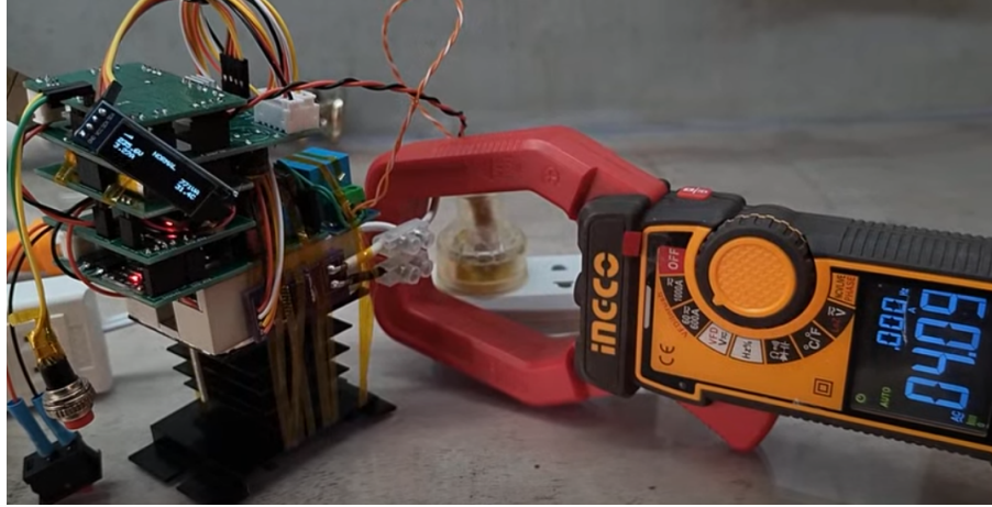
Figure 3.21. Data-collection setup for current calibration.
