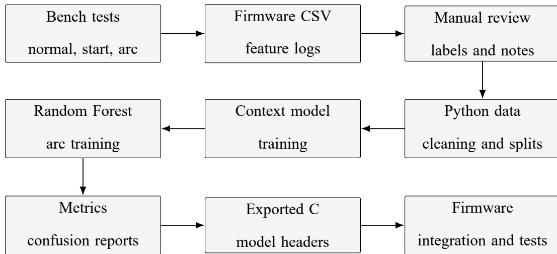
Figure 3.15. Data logging, labeling, and TinyML deployment workflow.
