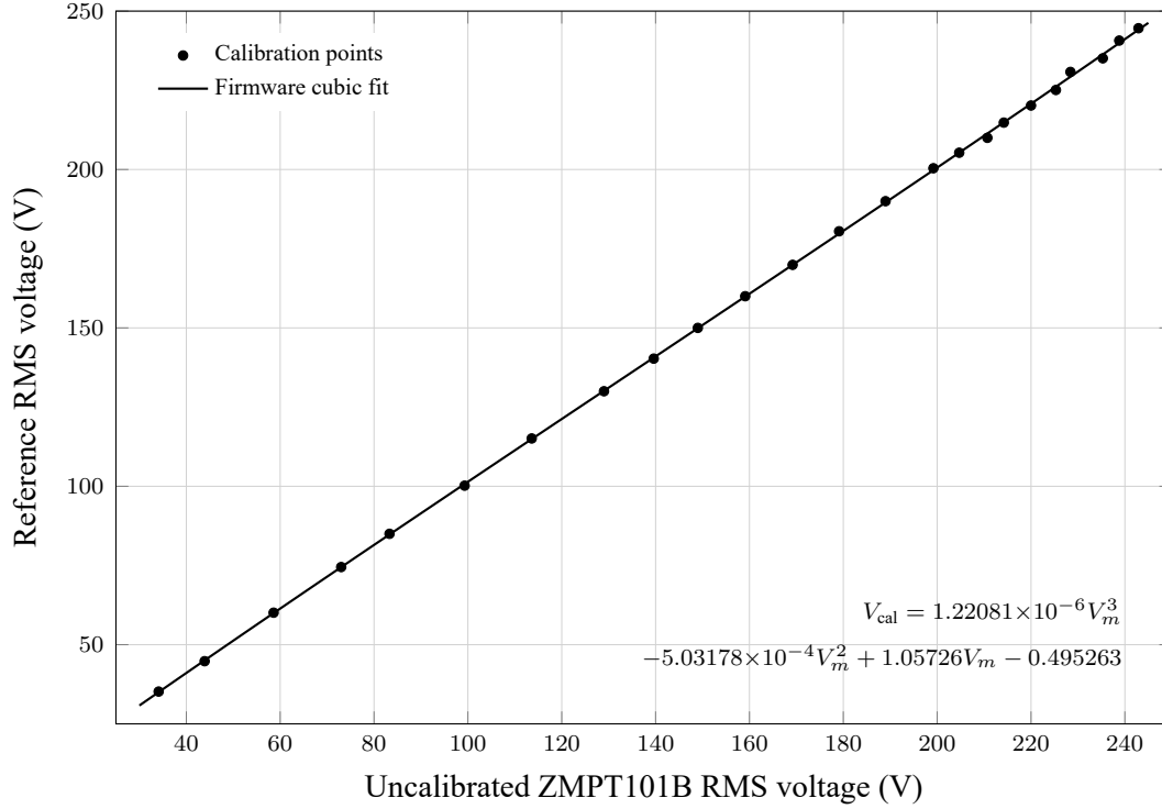
Figure 3.20. Cubic regression for voltage calibration.
