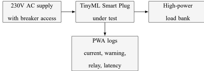
Figure 3.25. Testing setup block diagram for overload evaluation.
