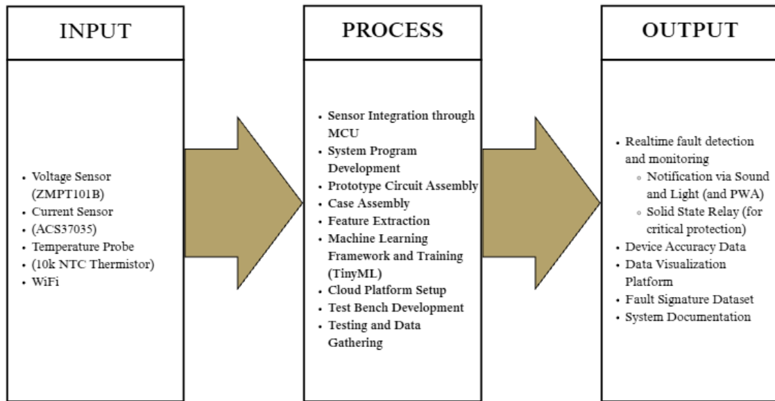
Figure 3.1. Conceptual framework of the TinyML Smart Plug.
