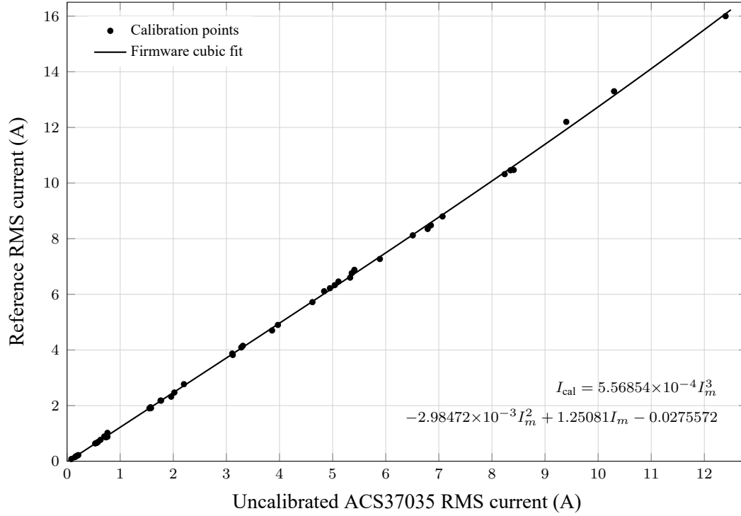
Figure 3.23. Cubic regression for current calibration.
