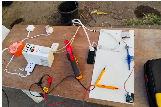
Figure 3.26. Actual test setup for overload evaluation.
