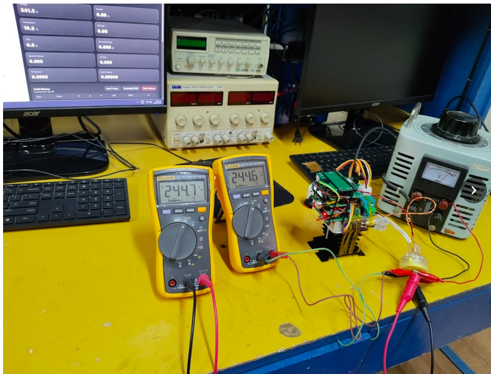
Figure 3.19. Data-collection setup for voltage calibration.
