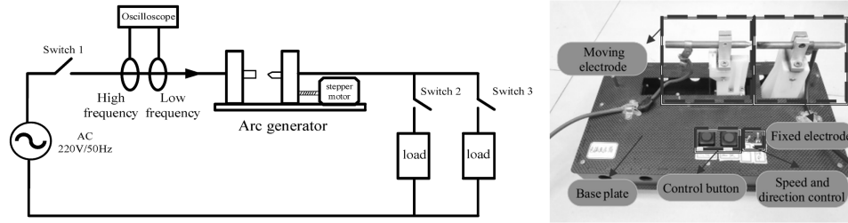
Figure 3.30. Series arc-fault test platform.
