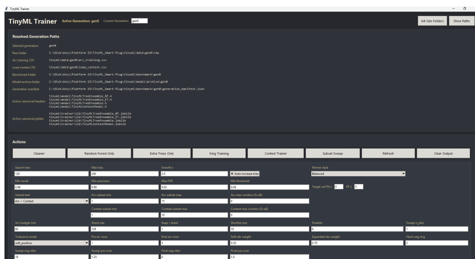
Figure 3.18. Local Python TinyML trainer.
