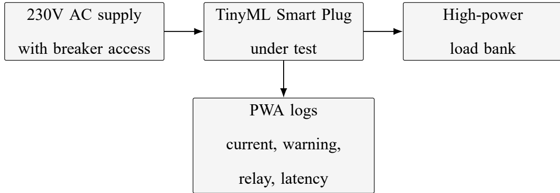
Figure 3.25. Testing setup block diagram for overload evaluation.
