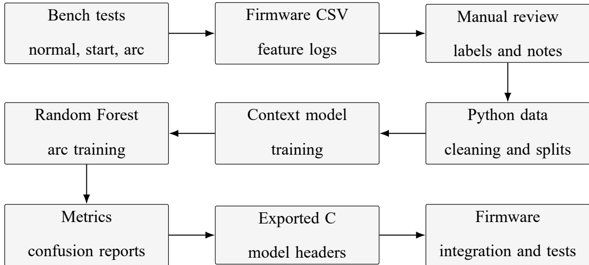
Figure 3.15. Data logging, labeling, and TinyML deployment workflow.
