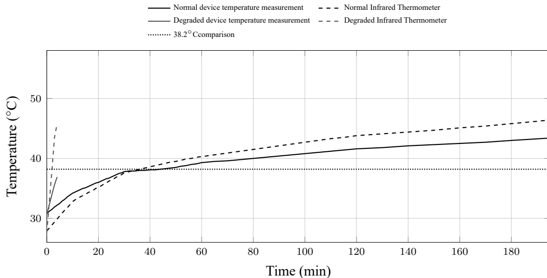
Figure 4.5. Water heater plus four halogen lamps temperature trend during characterization.
