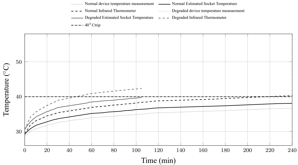
Figure 4.7. Water heater plus one halogen lamp trend during protection validation.
