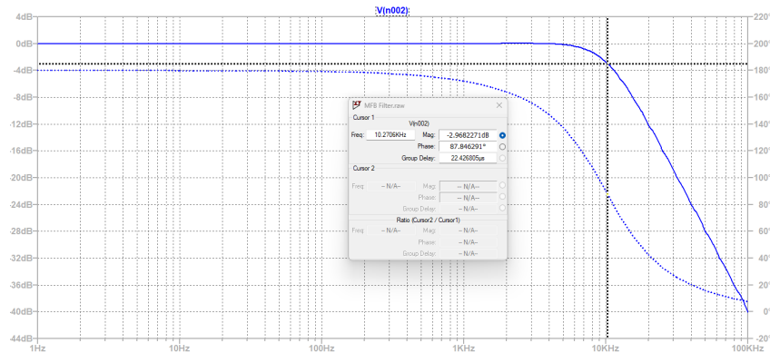
Figure 3.10. Bode response of the anti-aliasing filter.
