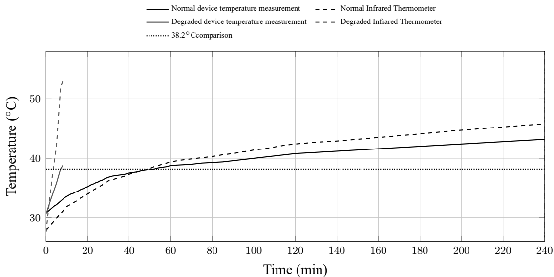
Figure 4.4. Water heater plus three halogen lamps temperature trend during characterization.
