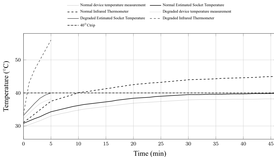
Figure 4.10. Water heater plus four halogen lamps trend during protection validation.
