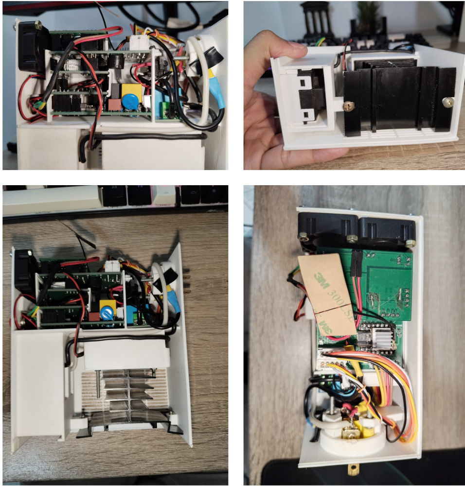
Figure 3.12. Actual prototype assembly without the case.
