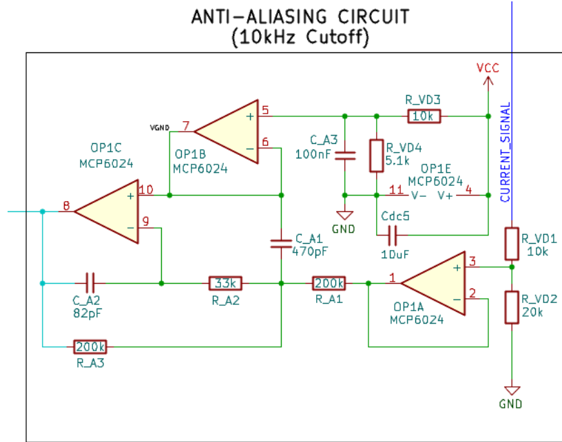
Figure 3.9. Second-order multiple-feedback low-pass anti-aliasing circuit.
