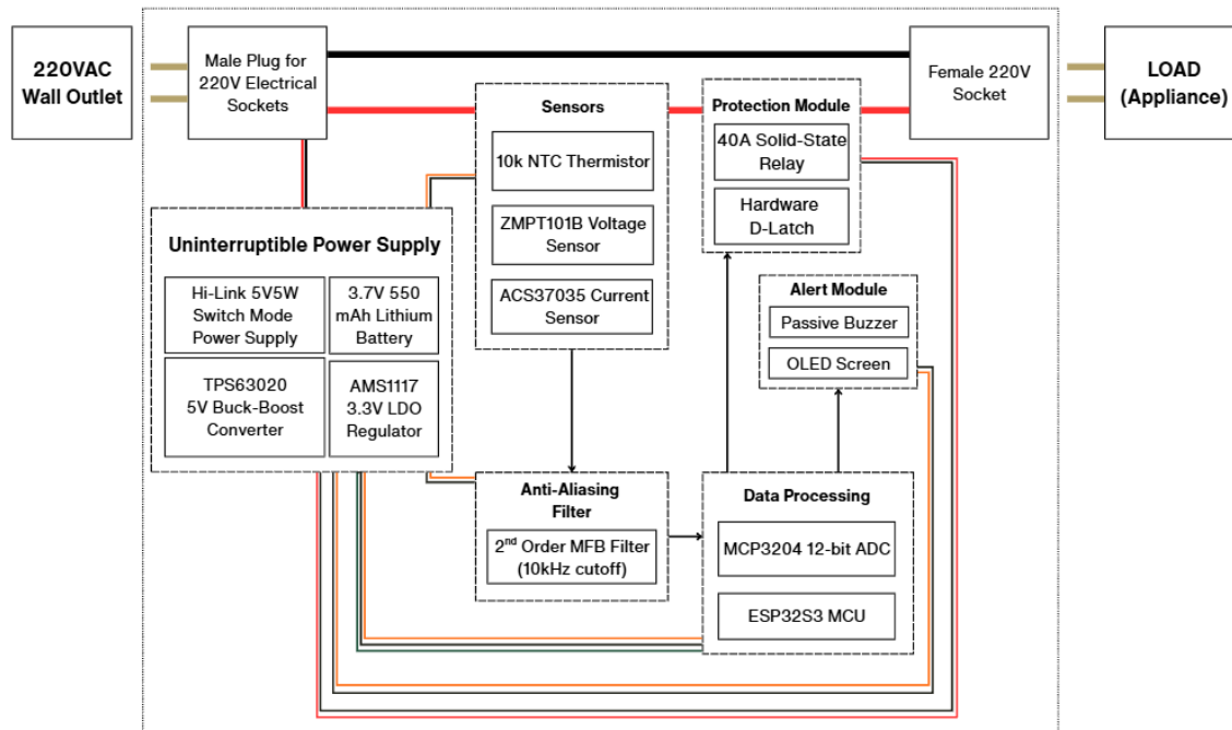
Figure 3.7. Block diagram of the prototype hardware.
