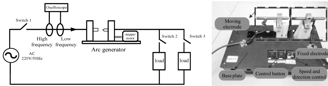
Figure 3.30. Series arc-fault test platform.
