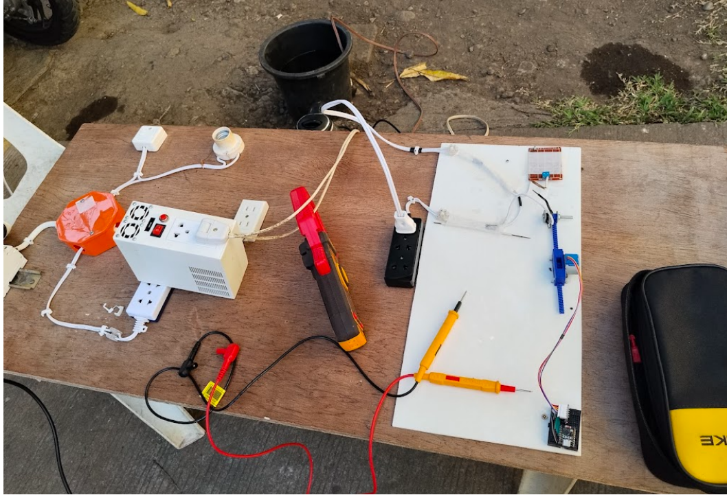
Figure 3.26. Actual test setup for overload evaluation.
