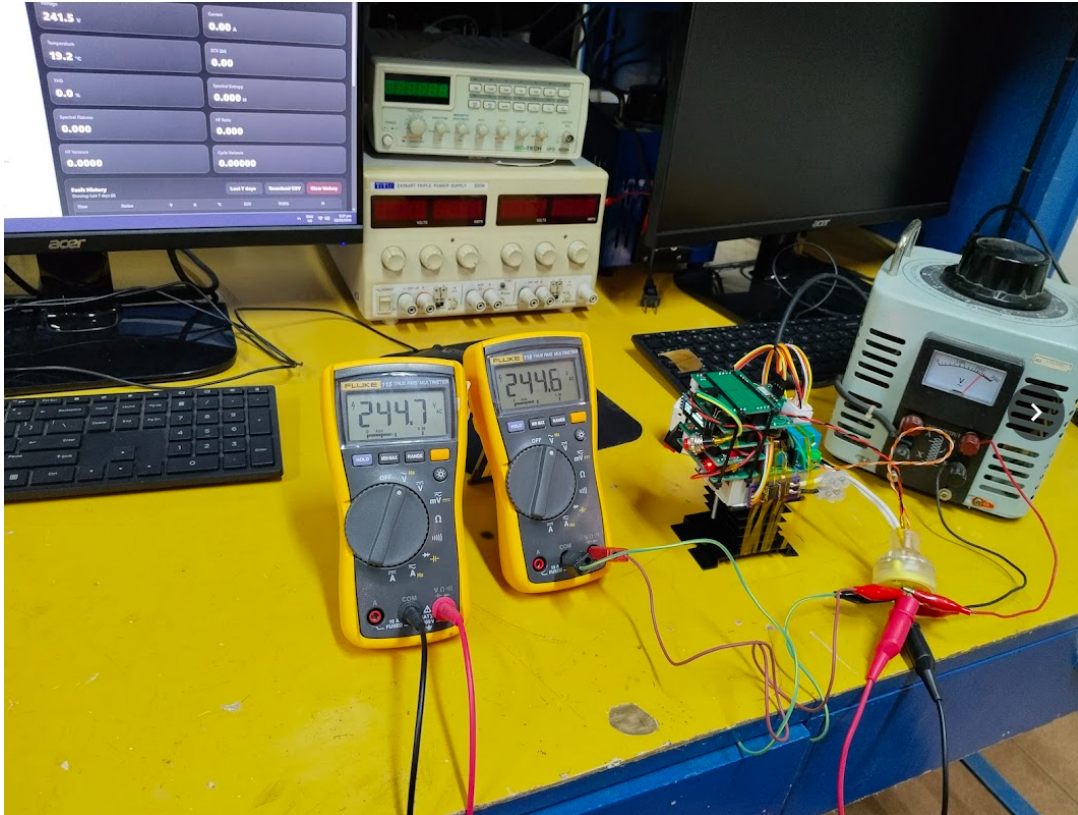
Figure 3.19. Data-collection setup for voltage calibration.
