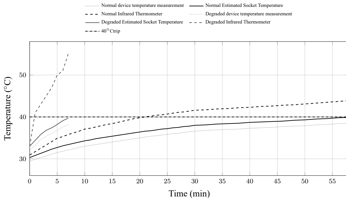
Figure 4.9. Water heater plus three halogen lamps trend during protection validation.
