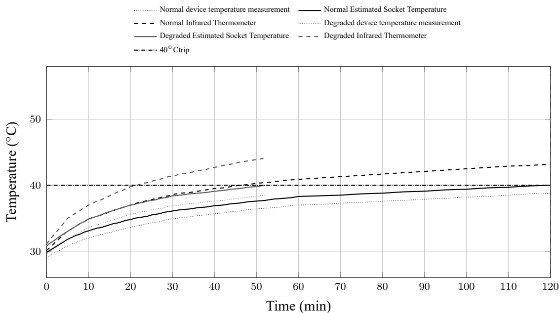
Figure 4.8. Water heater plus two halogen lamps trend during protection validation.
