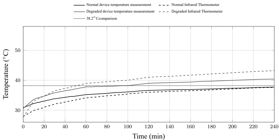
Figure 4.2. Water heater plus one halogen lamp temperature trend during characterization.
