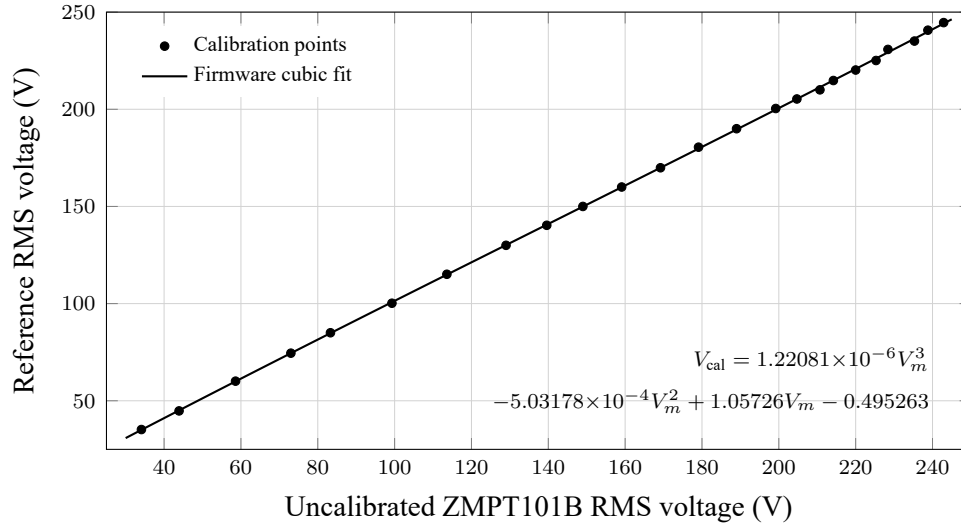
Figure 3.20. Cubic regression for voltage calibration.
