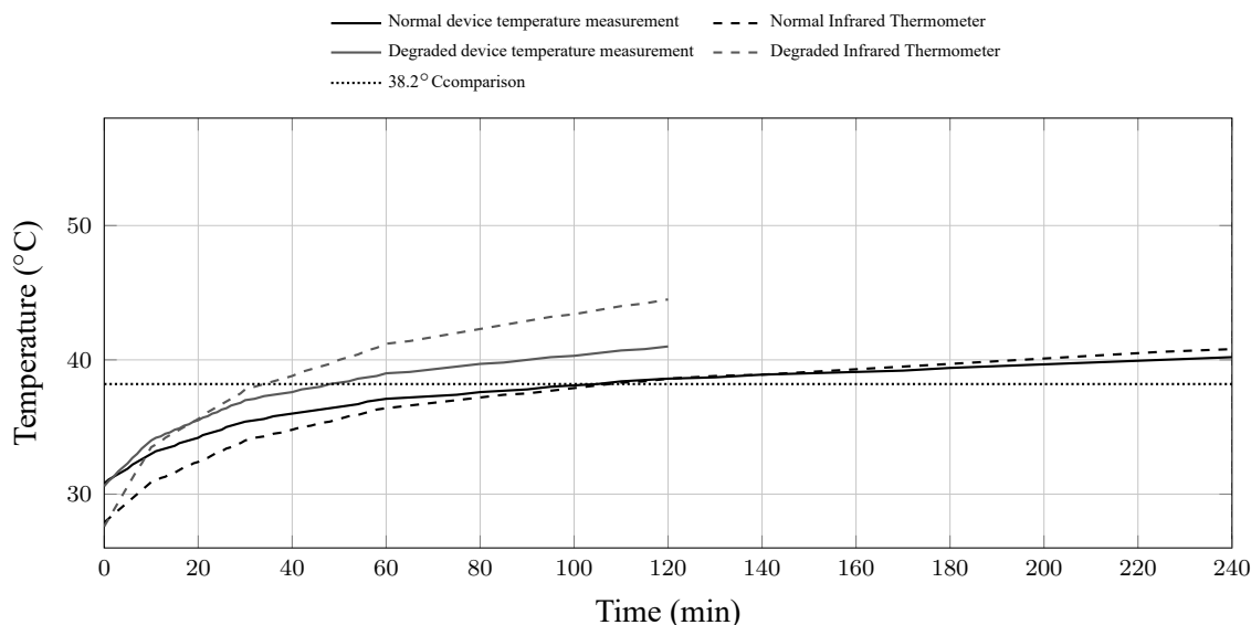
Figure 4.3. Water heater plus two halogen lamps temperature trend during characterization.
