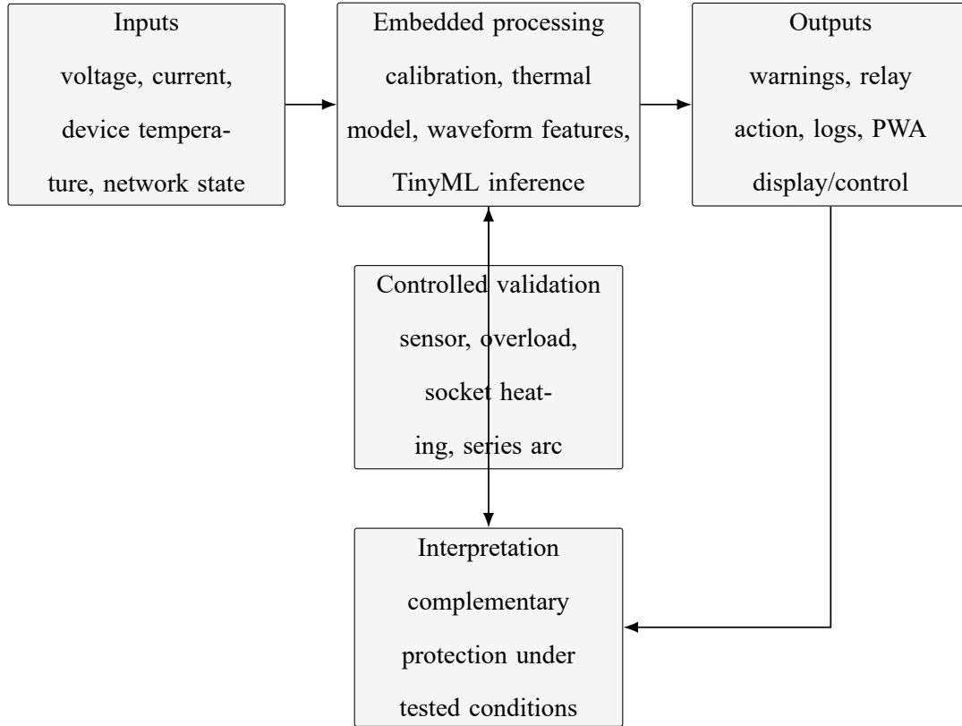
Figure 3.1. Conceptual framework of the TinyML Smart Plug.
