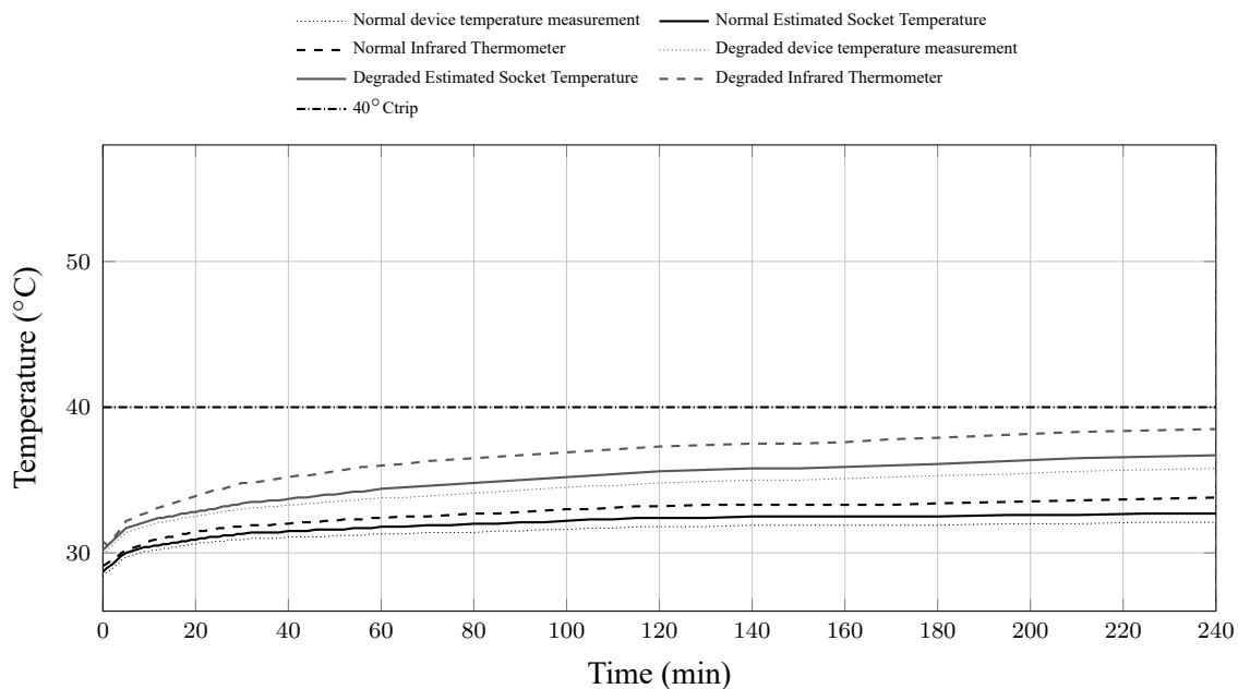
Figure 4.6. Water heater temperature trend during socket-heating protection validation.
