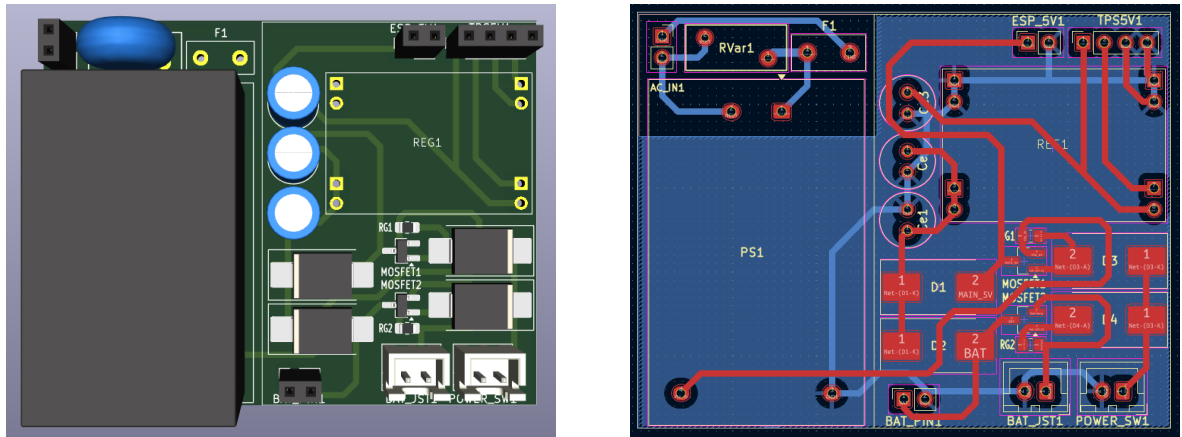
Figure B.1. PCB layout for the power-supply section.
