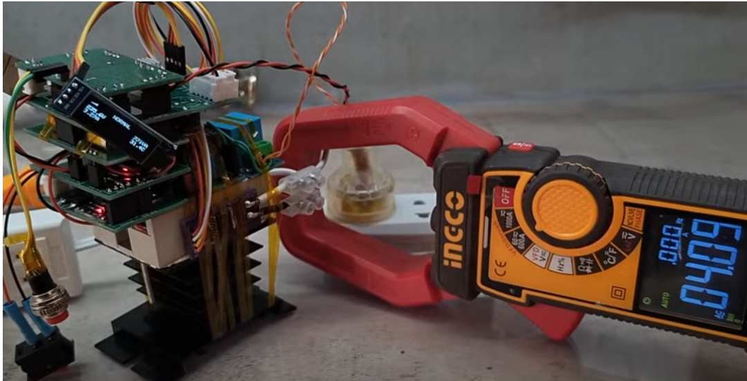
Figure 3.21. Data-collection setup for current calibration.
