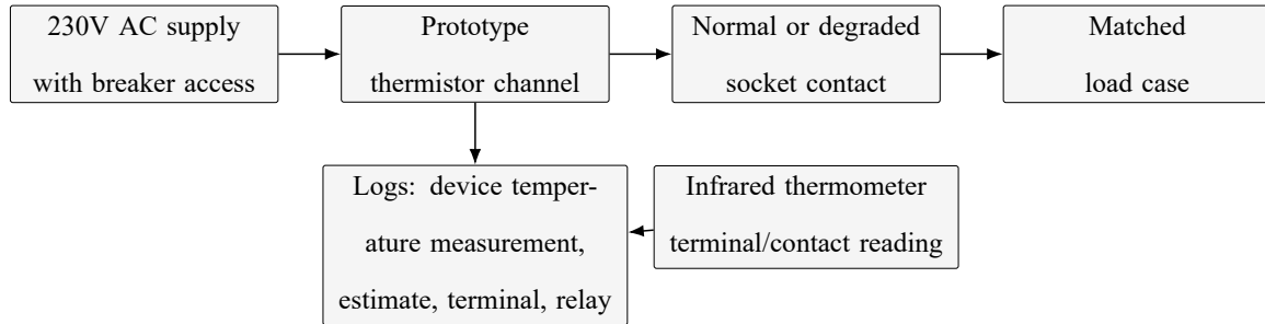
Figure 3.27. Testing setup block diagram for socket-heating evaluation.
