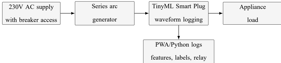
Figure 3.31. Testing setup block diagram for series arc-fault evaluation.
