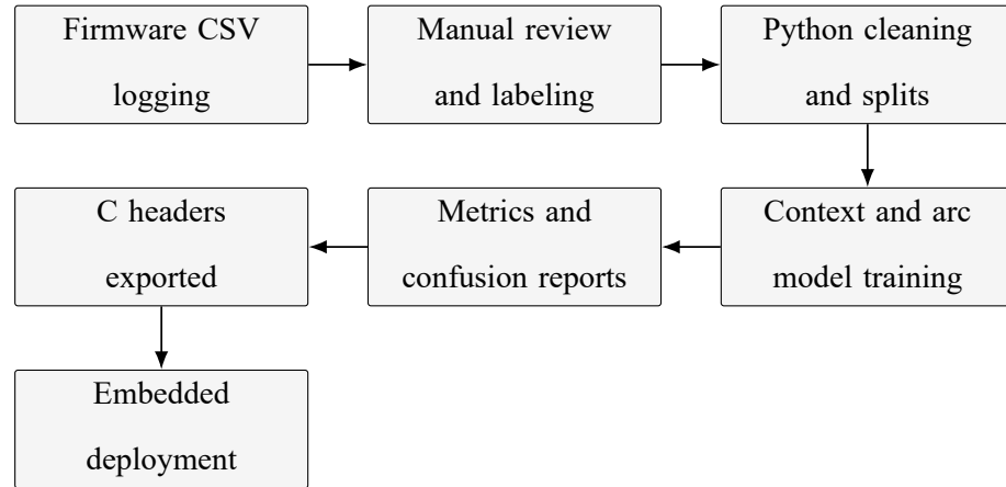
Figure 3.15. Data logging, labeling, and TinyML deployment workflow.
