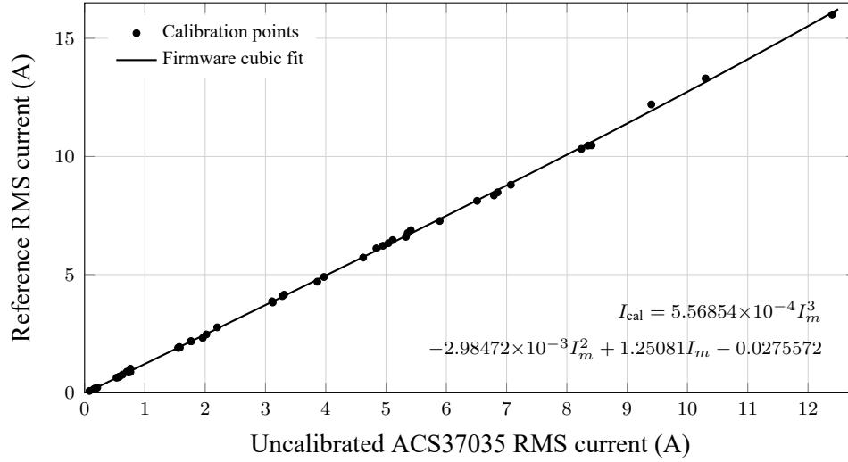
Figure 3.23. Cubic regression for current calibration.
