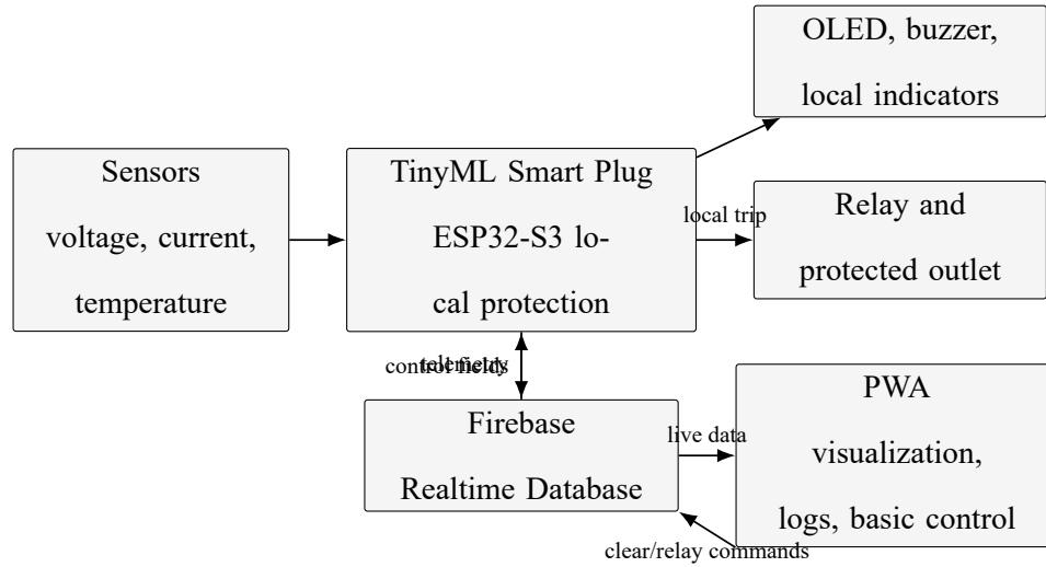
Figure 3.2. System architecture of the TinyML Smart Plug.
