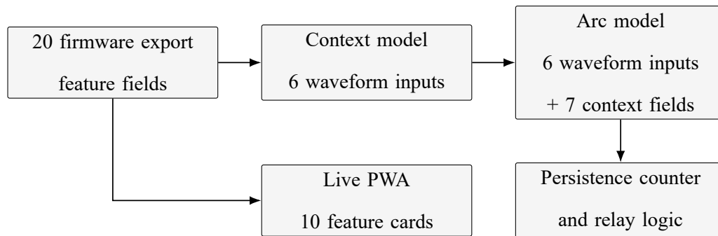
Figure 3.16. TinyML processing sequence from feature logging to embedded inference.
