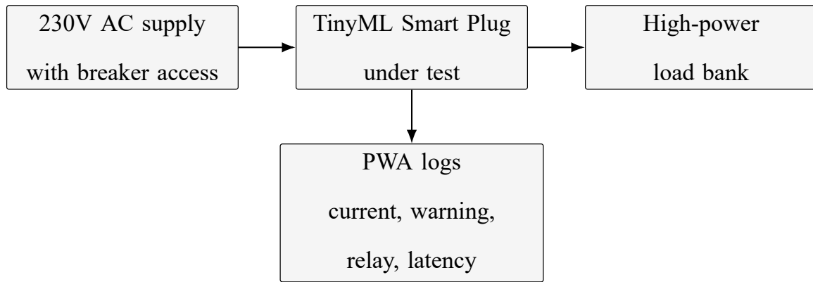
Figure 3.25. Testing setup block diagram for overload evaluation.
