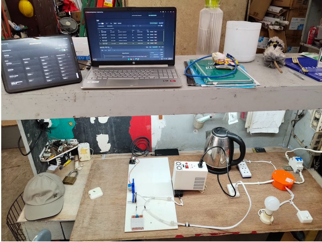
Figure 3.32. Actual test setup for series arc-fault evaluation.
