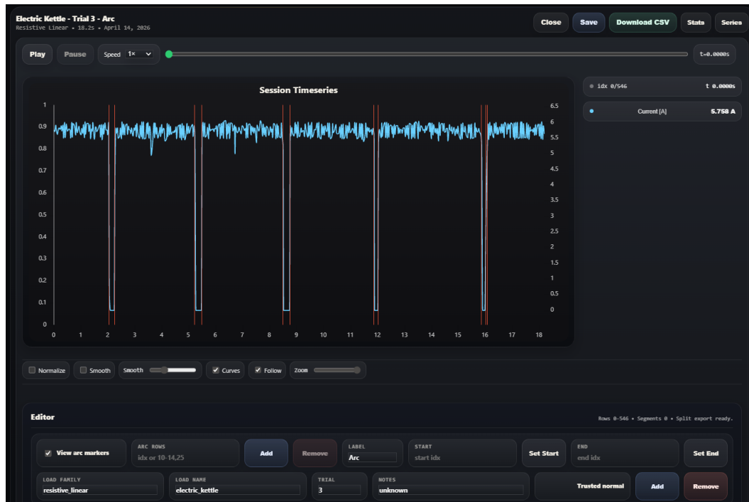
Figure 3.17. Arc labeling using logged waveform data.
