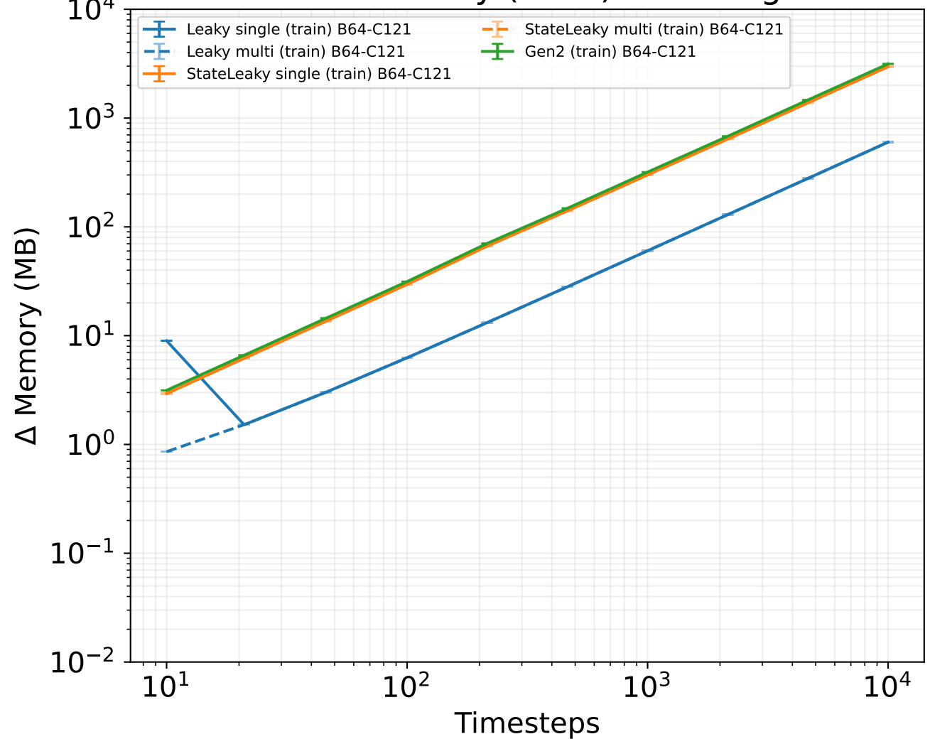
SNN Memory (Peak) - Training
