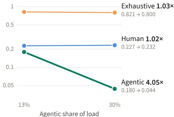
a Agentic share, 13% → 30%
