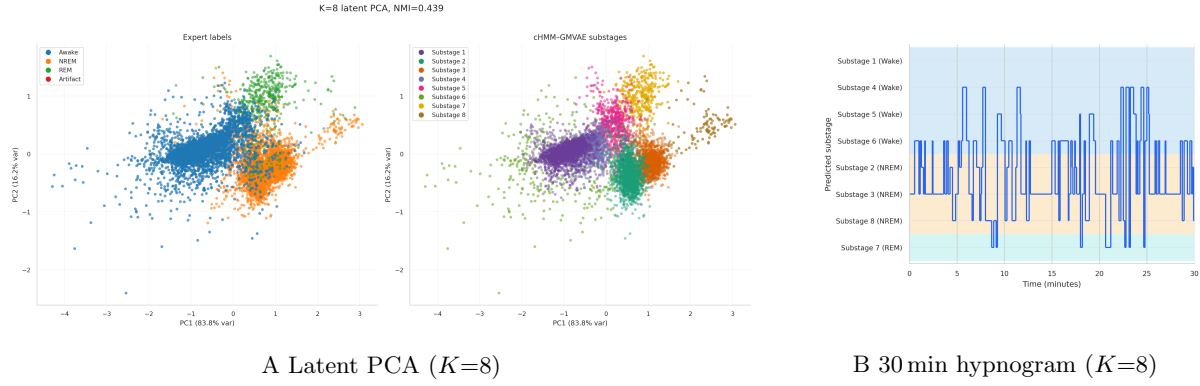
Fig 4. Latent separation and temporal structure at K=8 (population sweep, best seed). A , PCA of encoder means coloured by expert macro or predicted substage. B , Example 30 min hypnogram.
