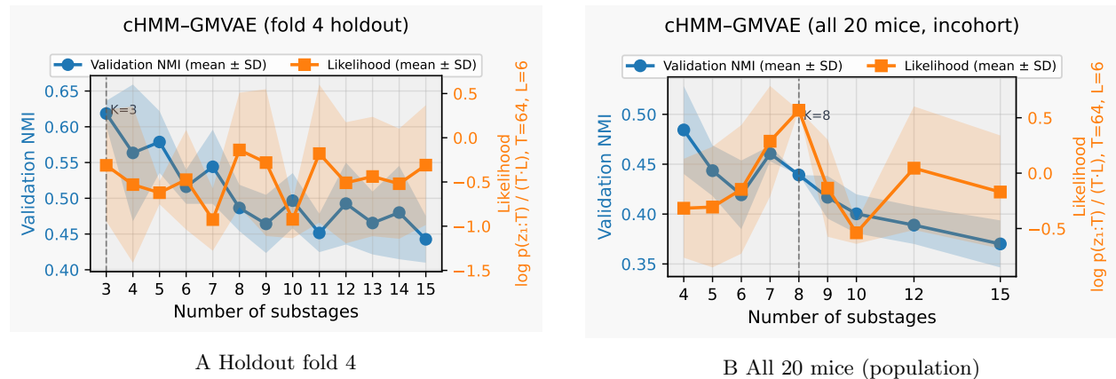
Fig 3. Substage resolution sweeps. Mean validation prior NMI (blue) and mean normalised prior log-density (orange) versus mixture count K . Shaded bands show mean \pm SD across seeds. A , Holdout fold 4 (six mice, K=3-15 ). B , Population cohort (twenty mice). Prior log-density peaks at K=8 on panel B.
