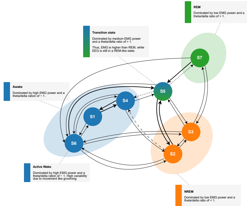
Fig 6. K=8 substate organisation (best seed; S8 omitted). Nodes mark substates in latent space (Fig 4A). Edges from Appendix D.1 with p > 0.05 . Solid colours mark stable Wake, NREM, and REM substates. Gradients mark transition substates.
