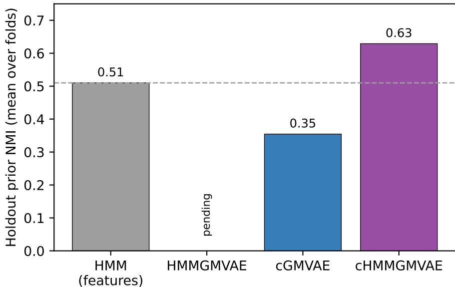
Joint cross-lab holdout (locked recipes)
