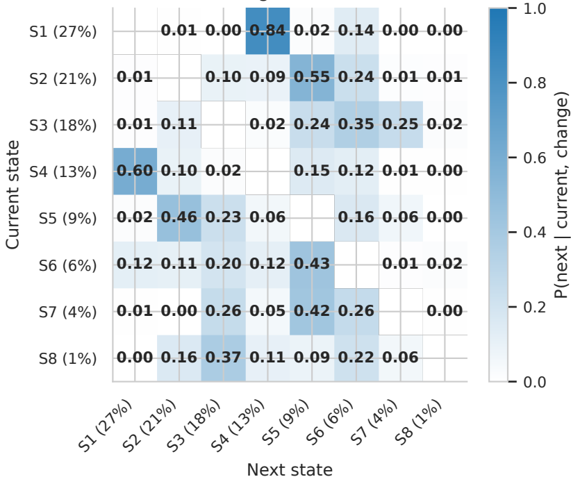
Substage transitions
