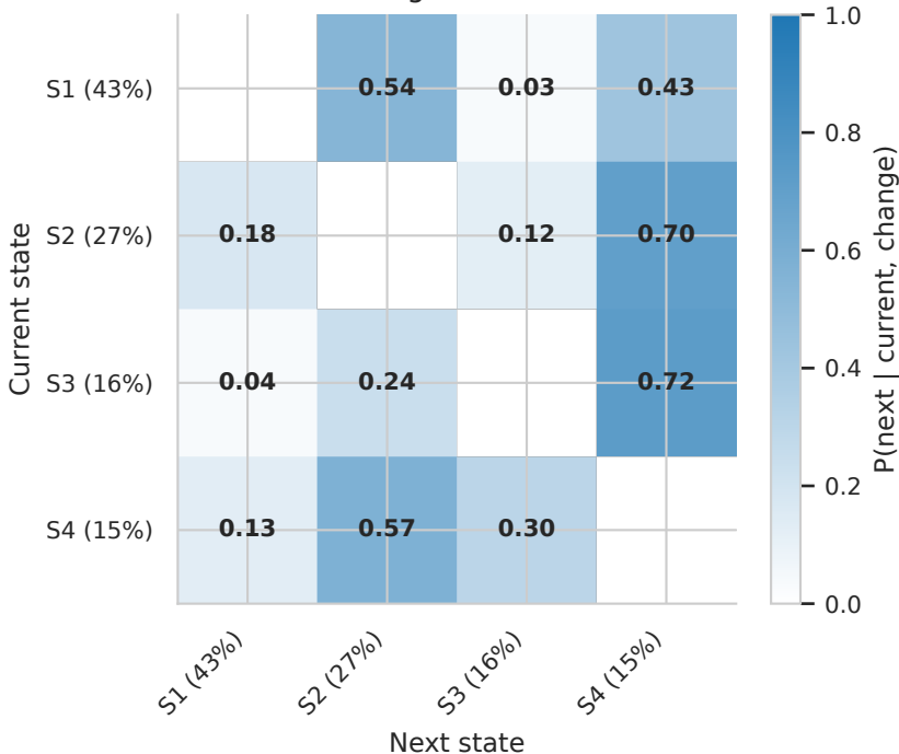
Substage transitions
