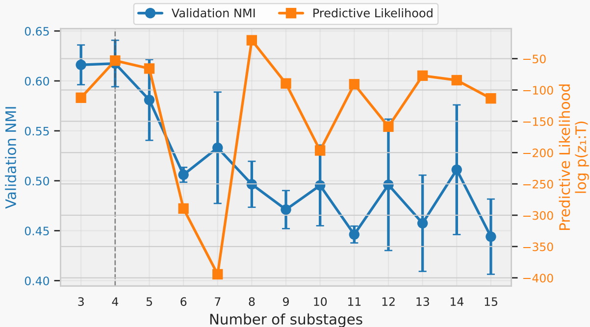
cHMM-GMVAE (fold 4 holdout)
