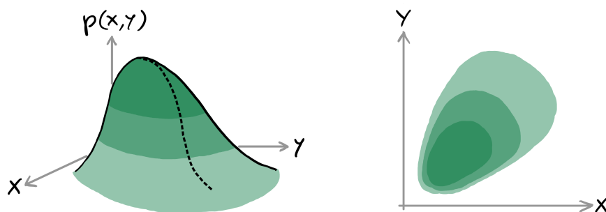
Figure 12: A two-variable joint probability distribution p(x, y) visualised as a 3D figure (left) and as a 2D colour map (right)
