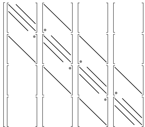
Figure 26: Example of the structure of non-zero elements in the matrices A and B in the Crank-Nicolson scheme for 2+1 dimensions
