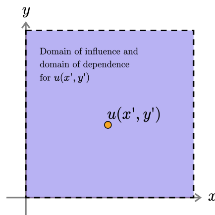
Figure 19: Domain of influence and domain of dependence for the solution at u(x', y') , given an elliptic PDE.
