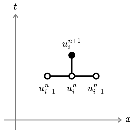
Figure 20: The computational stencil for the forward difference scheme in 1+1 dimensions
