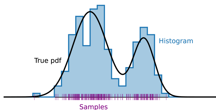
Figure 16: A set of samples, the corresponding histogram and the true pdf
