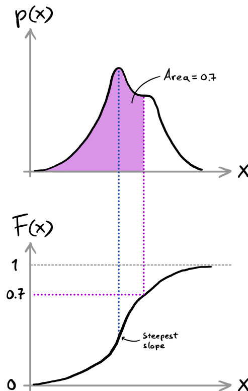
Figure 11: Illustration of the relation between a pdf p(x) and the corresponding cdf F(x)
