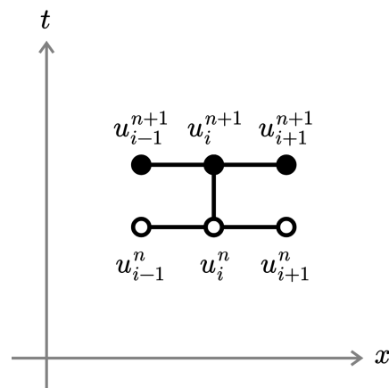
Figure 22: The computational stencil for the Crank-Nicolson scheme in 1+1 dimensions
