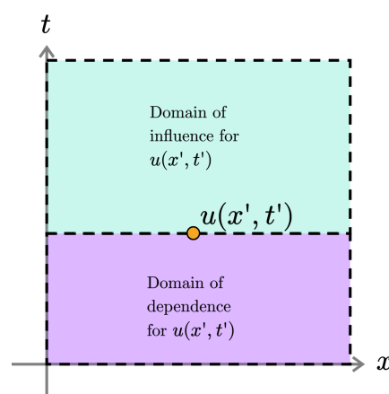
Figure 18: Domain of dependence and domain of influence for the solution at u(x', t') , given a parabolic PDE.
