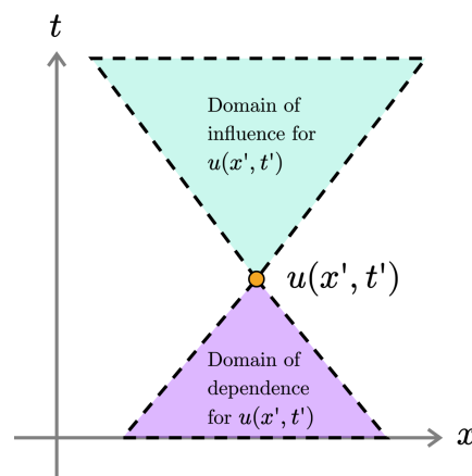
Figure 17: Domain of dependence and domain of influence for the solution at u(x', t') , given a hyperbolic PDE.
