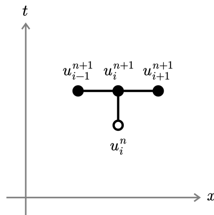
Figure 21: The computational stencil for the backward difference scheme in 1+1 dimensions
