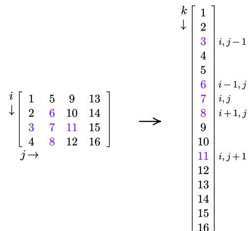
Figure 25: Example of how going from a 2D representation (with two indices i and j ) to a 1D representation (with index k ) breaks apart pairs that were neighbours in the 2D representation
