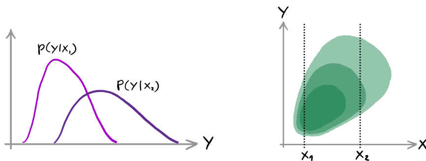
Figure 13: Two conditional probability distributions p(y|x_1) and p(y|x_2) (left), both derived from the joint distribution p(x, y) (right)
