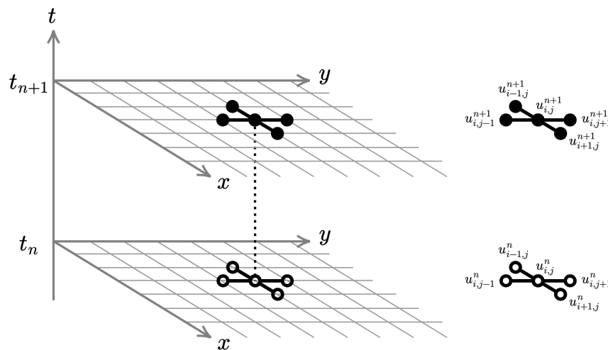
Figure 24: The computational stencil for the Crank-Nicolson scheme in 2+1 dimensions
