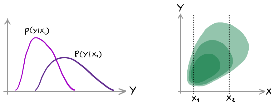
Figure 13: Two conditional probability distributions p(y|x_1) and p(y|x_2) (left), both derived from the joint distribution p(x, y) (right)
