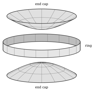
Figure 10: The three electrodes of a Penning trap: two end caps and a ring.
