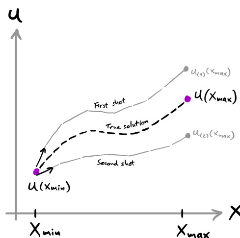
Figure 5: Sketch of the shooting method
