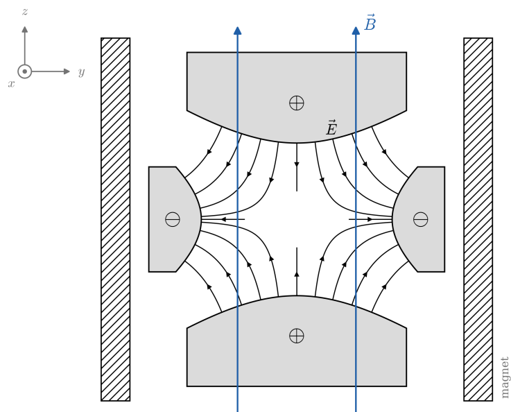
Figure 11: Cross section of a Penning trap. The end caps (top and bottom) are held at a positive potential and the ring (left and right) at a negative potential, giving the electric field lines shown in black. The whole trap sits inside a magnet, which sets up a homogeneous magnetic field \vec{B} in the z direction.
