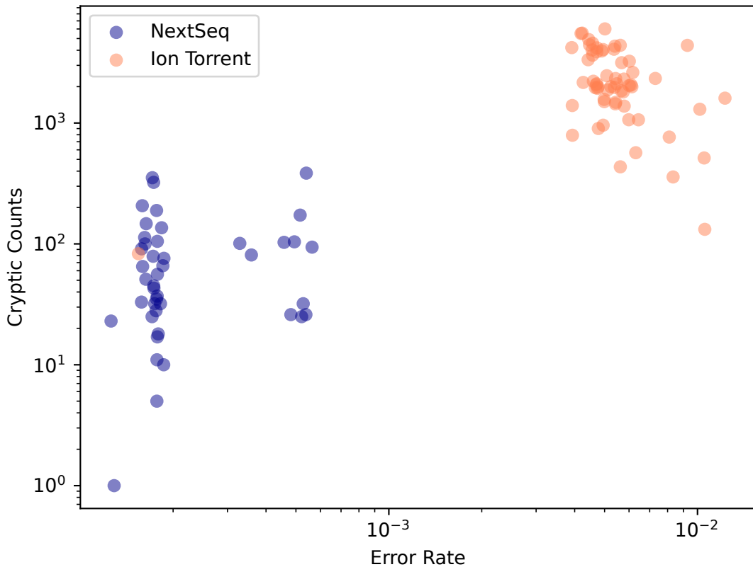
Cryptic Counts vs Sequencing Error Rate
