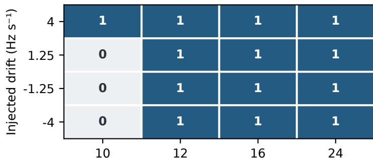
All three ON (active indices [0, 2, 4]) Intrinsic width: 1 channel
