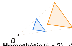
Homothétie ( k = 2 ) : z' = 2z - \omega
