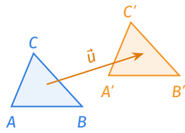
Translation : z' = z + b
