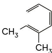
ortho-xylène (1,2)
