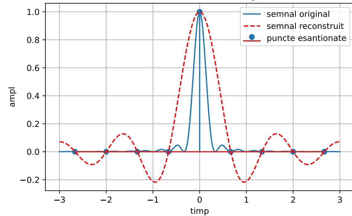
B = 3, fs = 2 (aliasing)
