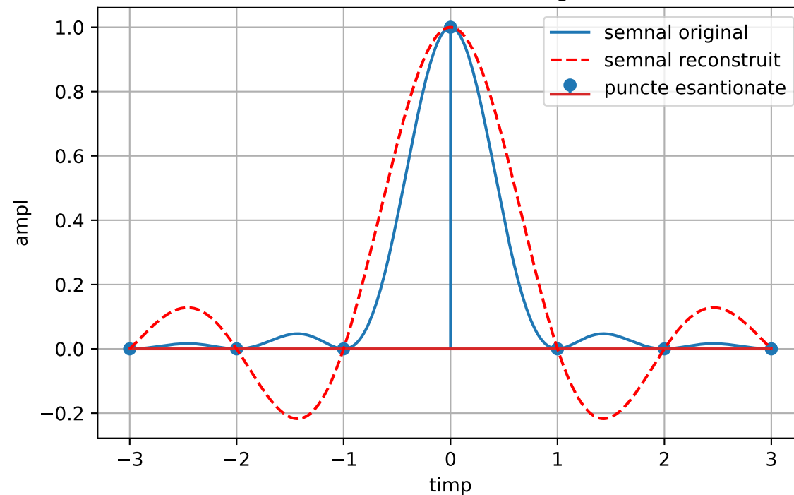
B = 1, fs = 1.5 (aliasing)
