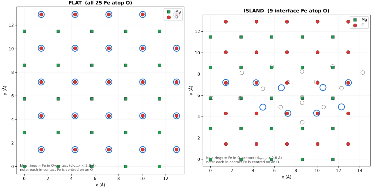
Figure S3: Top view of the interface, showing the metal atoms registered directly above the substrate oxygen on the MgO(001) lattice.
