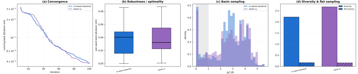
Figure S6: The same four panels for the dipole family.
