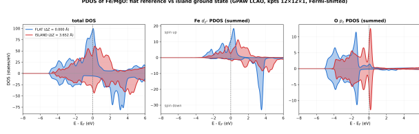
Figure S2: Total DOS, Fe- d_{z^2} and O- p_z for the flat monolayer (blue) and the island ground state (red).
