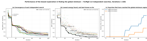
Figure S1: Best-so-far \Delta E/N against iteration for each of the 13 searches, with the median over searches in black; (b) the lowest energy found in each iteration (points) and the best-known energy across all searches (black line), with the iterations at which it first crosses 0.20, 0.10, 0.05, 0.02 and 0.005 eV/atom marked; (c) the fraction of searches whose own best-so-far has come within 0.05 and 0.02 eV/atom of the global minimum. The vertical line in each panel marks iteration 10, where relaxation begins.
