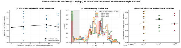
Figure S8: (a) the flat-basin minimum against the constraint, pooled per arm with the individual searches overlaid; (b) the \Delta Z distributions of each arm; (c) the search-to-search spread within each arm.
