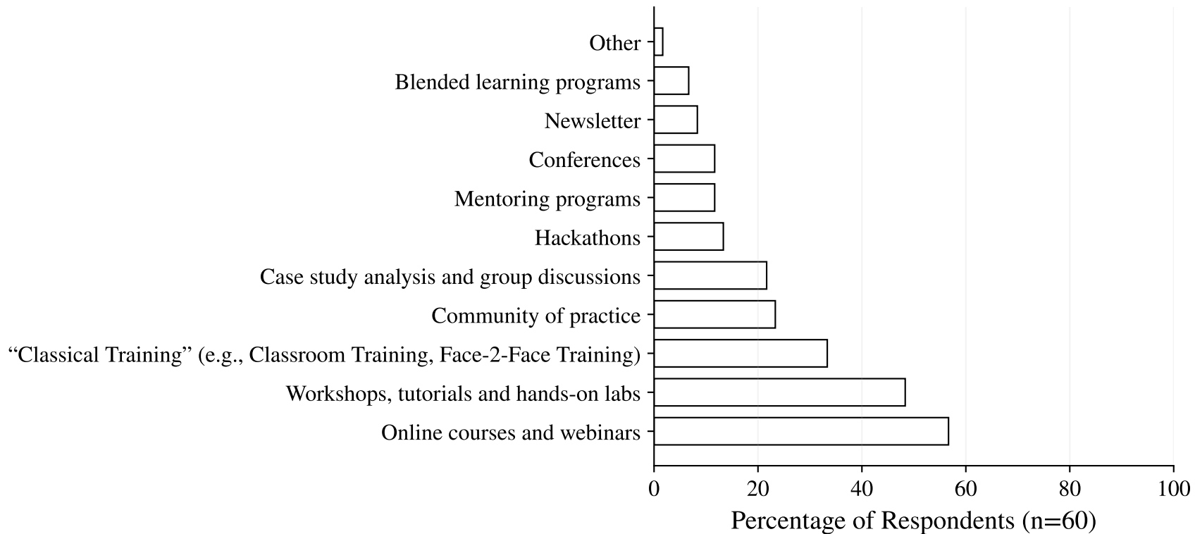
Training Format
