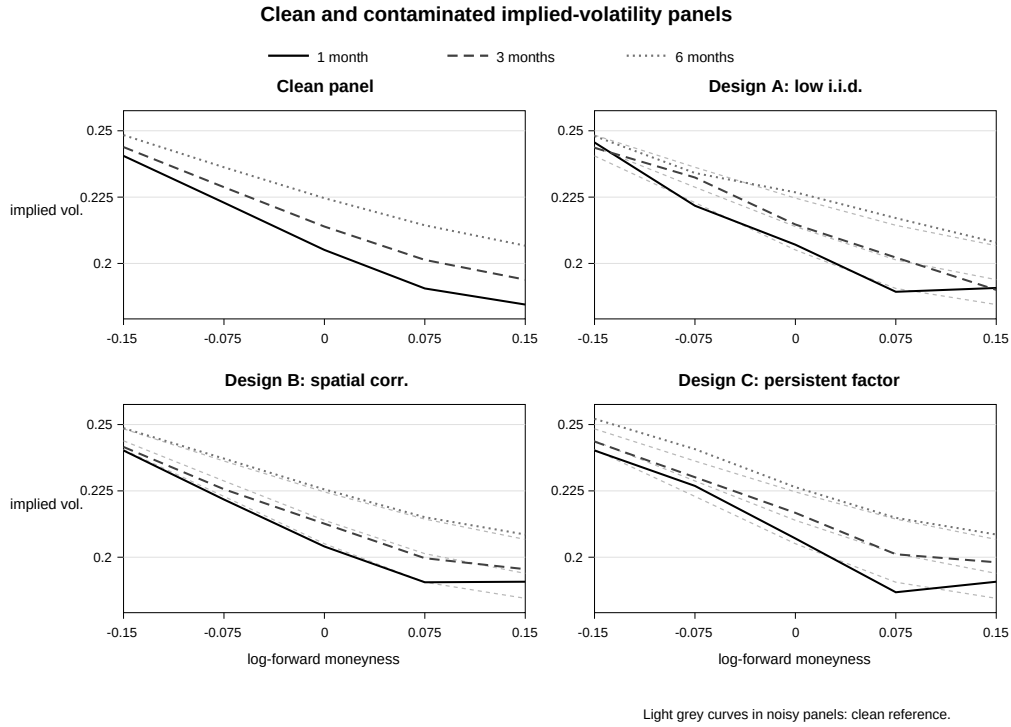
Figure 1: Clean and noisy implied-volatility panels for sample 000 at week index 129. The clean panel is generated exactly from the Heston pricing model. Designs A–C introduce increasingly structured quote distortions in implied-volatility space before prices are reconstructed and projected into admissible price intervals.
