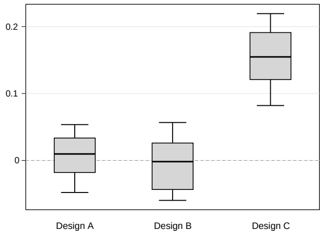
First-order autocorrelation
