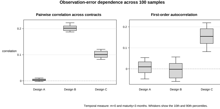
Figure 2: Dependence in the observation errors across the 100 samples. For each sample, the left panel averages the pairwise correlations between the error series for the 15 contracts. The right panel reports the first-order autocorrelation of the error series for the at-the-money three-month contract. Each box summarises the resulting sample-level values; the centre line is the median and the whiskers show the 10th and 90th percentiles.
