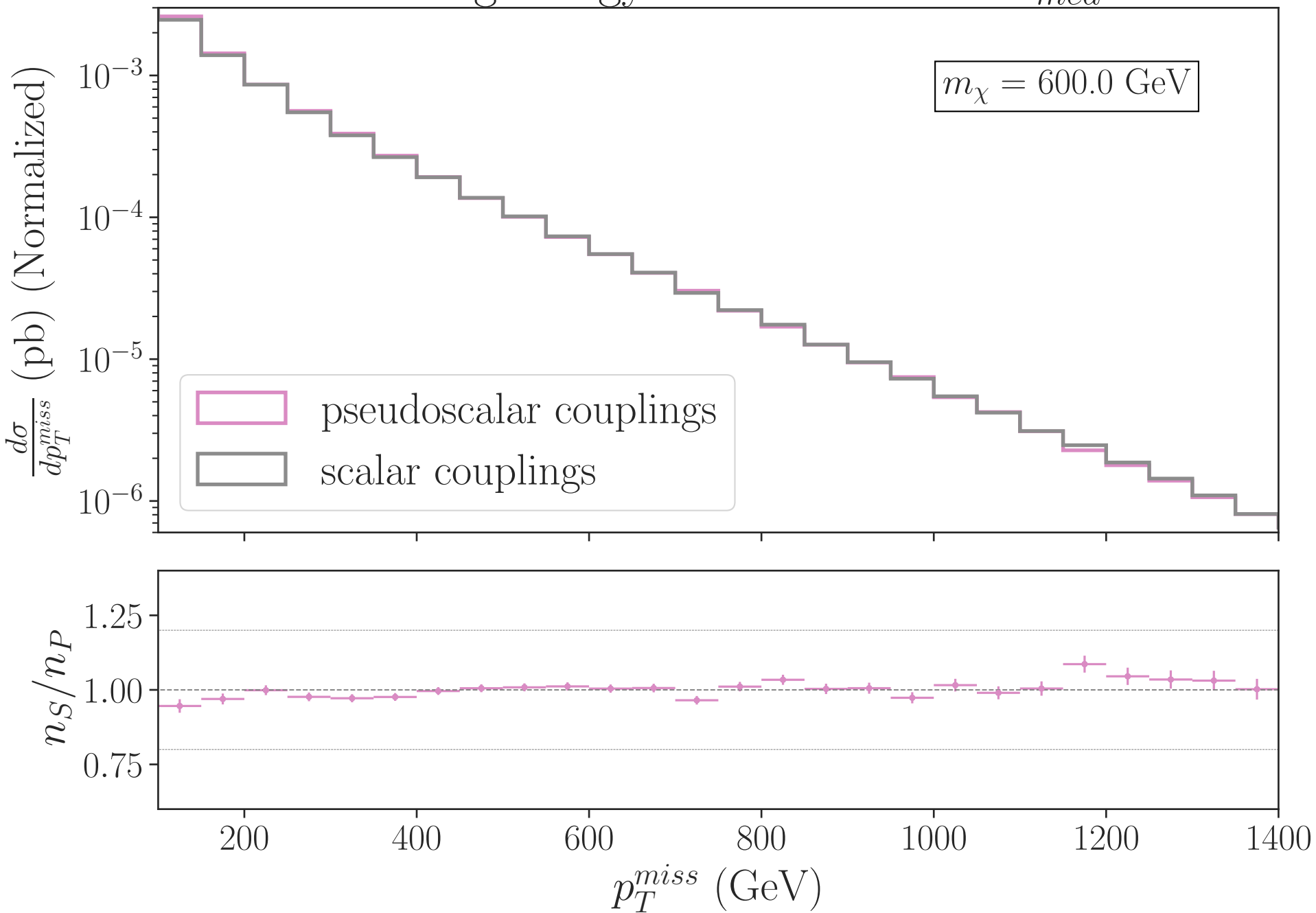
Mediator missing energy distribution for M_{med} = 1 TeV
