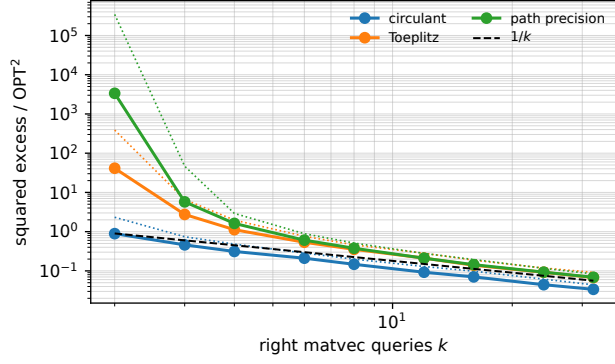
Figure 1: Relative squared excess for three 32 \times 32 families. The dashed line has slope 1/k .
